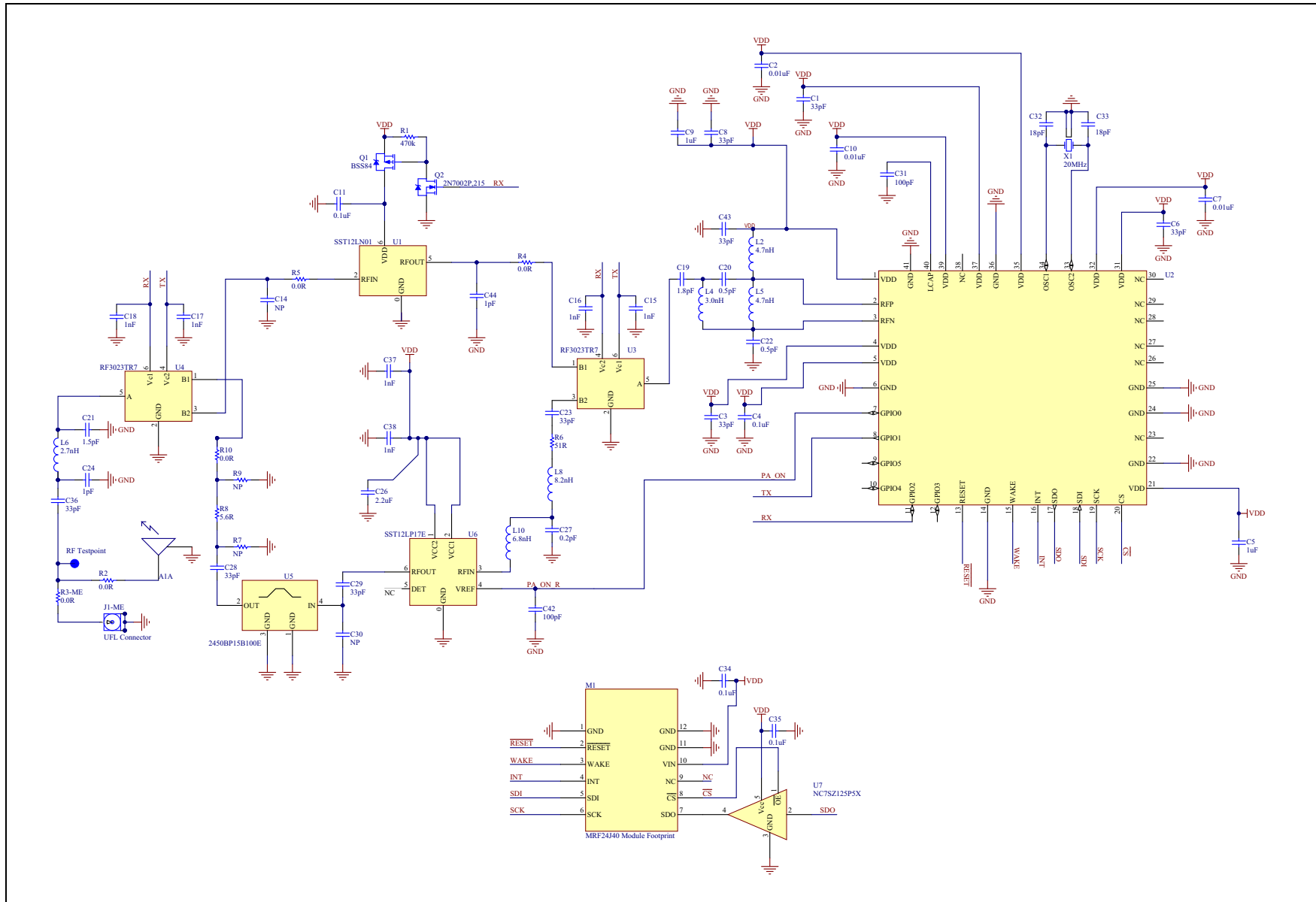
FIGURE 2-5: MRF24J40MD/ME SCHEMATIC
