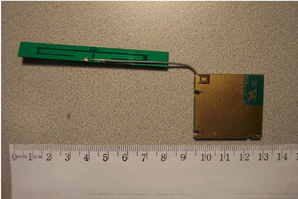
MC55i Wireless Module rear view
