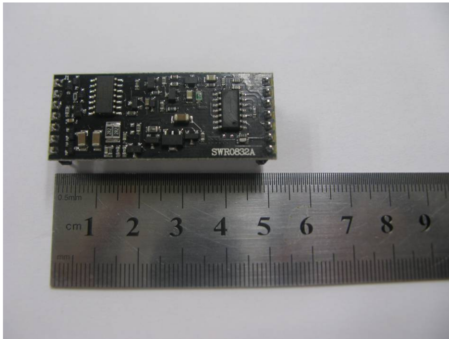
EUT – Switch Board Components View 2
