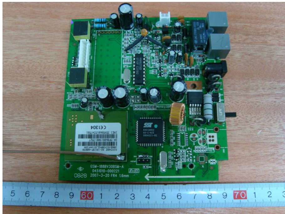
EUT – Main Board Components View 2
