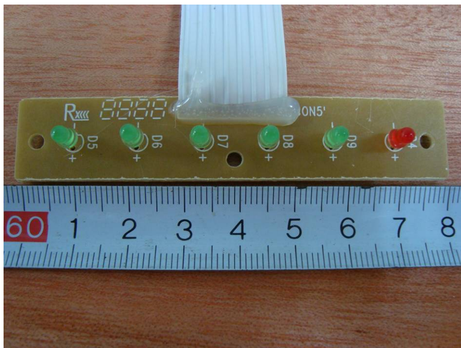
EUT – LED Board Components View
