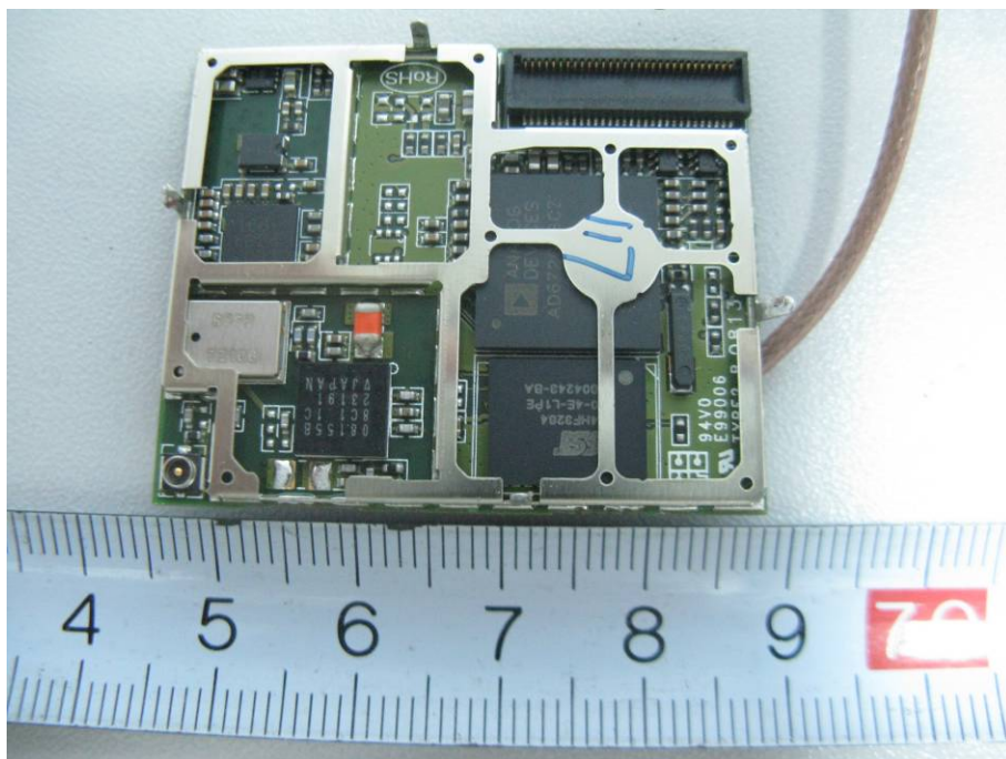
EUT – Module Cover off View
