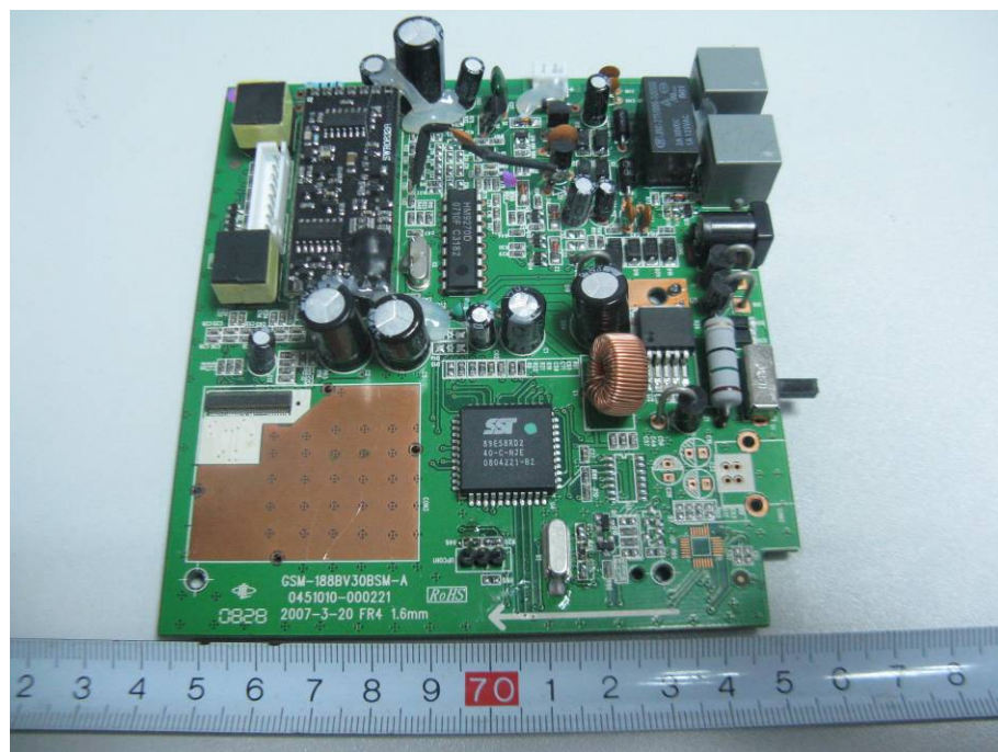
EUT – Main Board Components View 3
