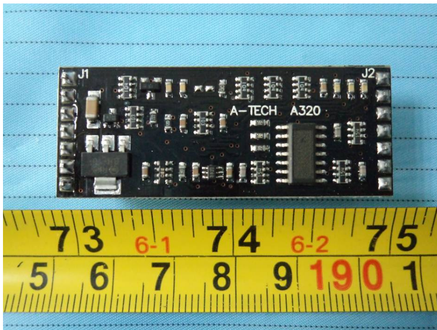
EUT – Auxiliary-1 Board Bottom View
