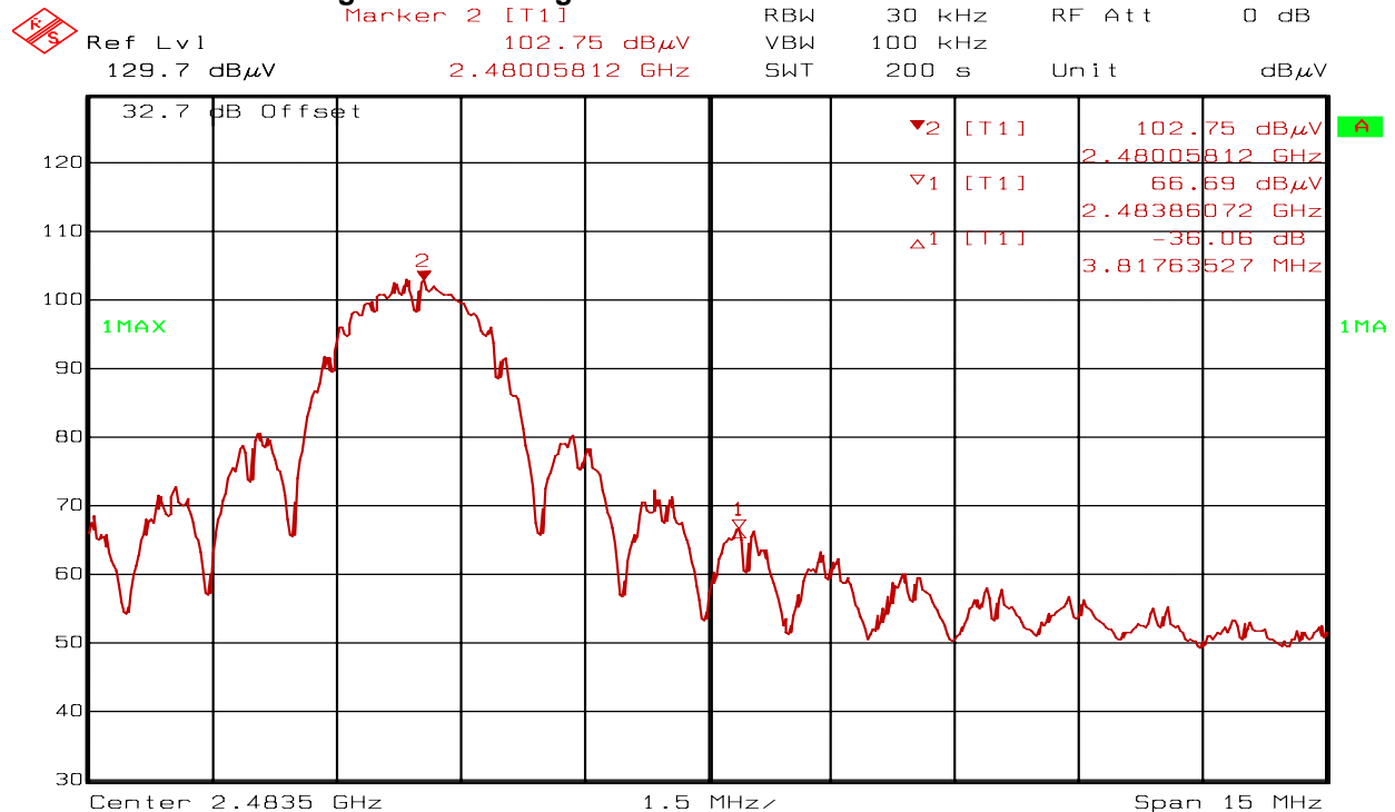
Figure 30 High Channel Marker Delta Measurement
