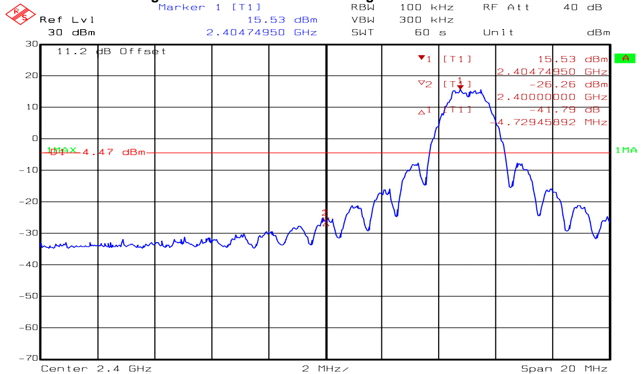
Figure 23 Conducted Band edge Measurement Ch11
