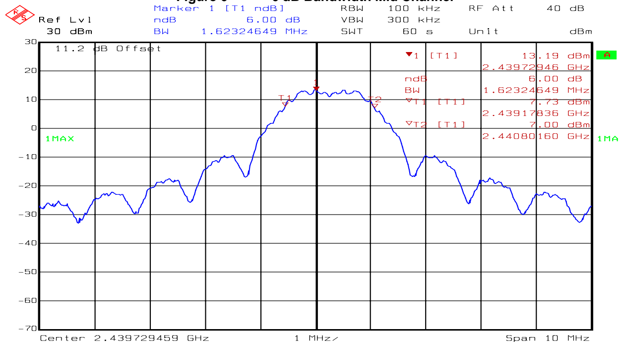
Figure 6 6 dB Bandwidth Mid Channel
