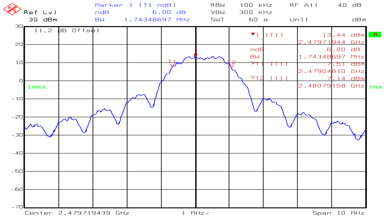
Figure 7 6 dB Bandwidth High Channel
