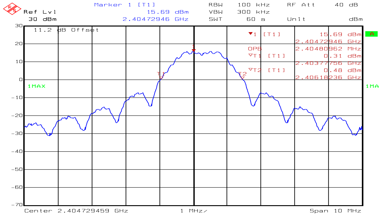
Figure 8 Occupied Bandwidth Low Channel
