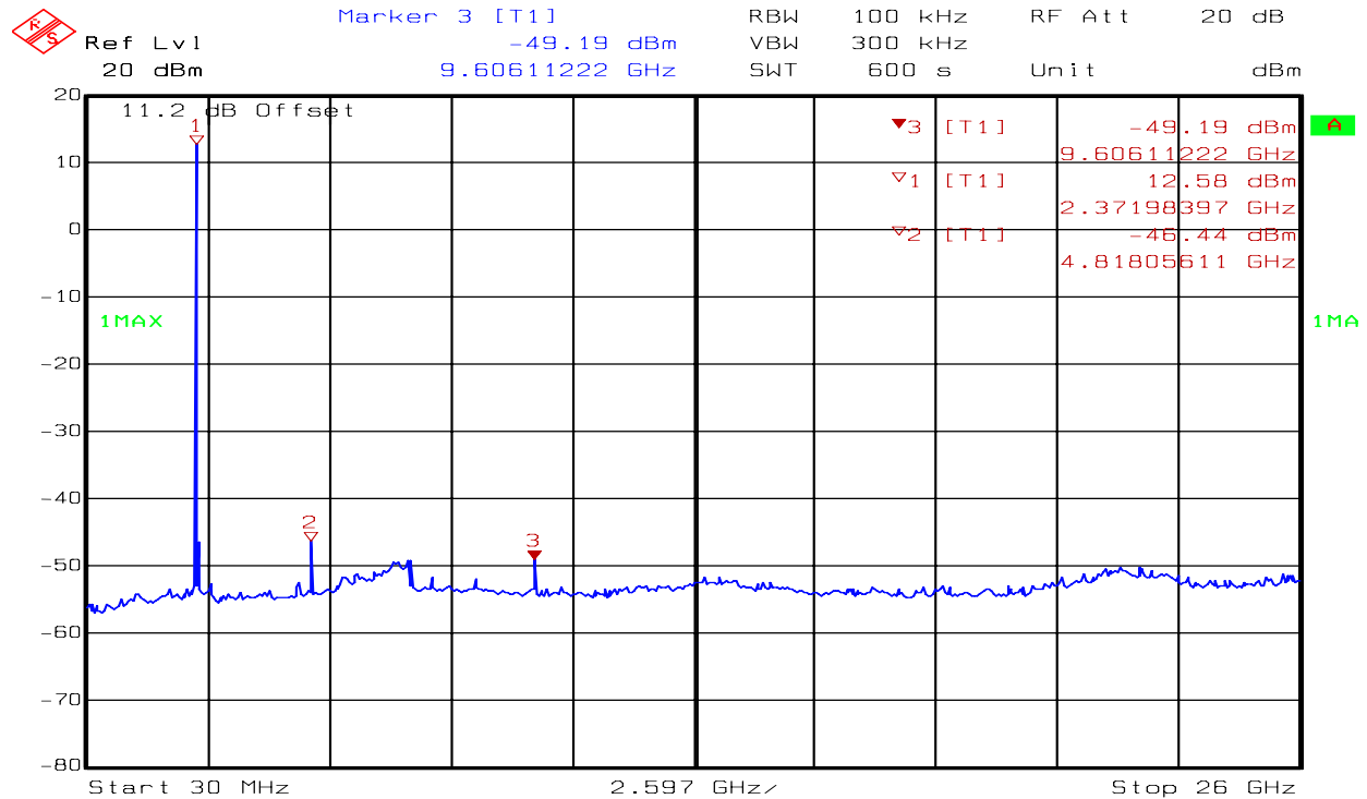
Figure 20 Conducted Spurious Ch11
