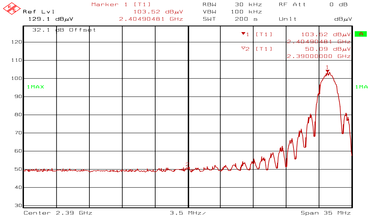
Figure 27 Low Channel Marker Delta
