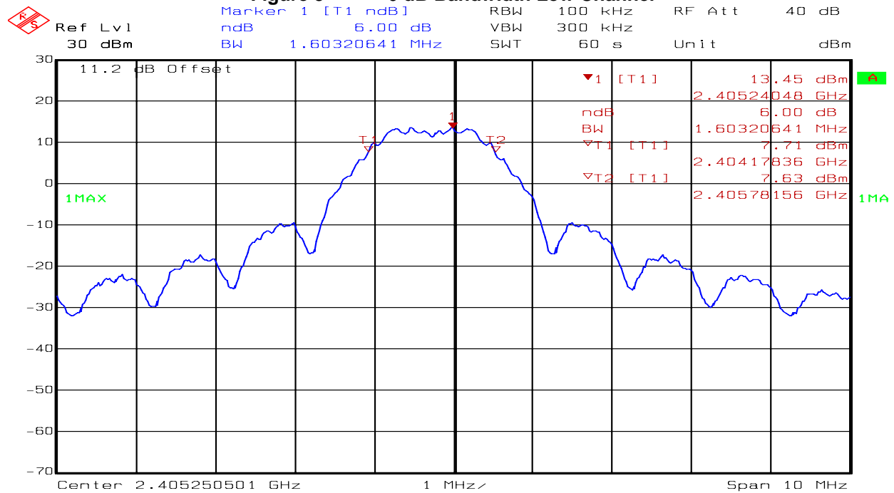
Figure 5 6 dB Bandwidth Low Channel
