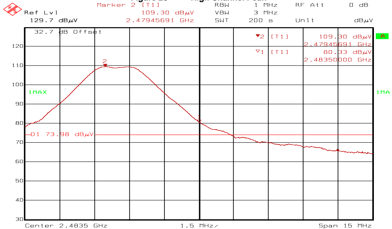
Figure 28 High Channel Peak
