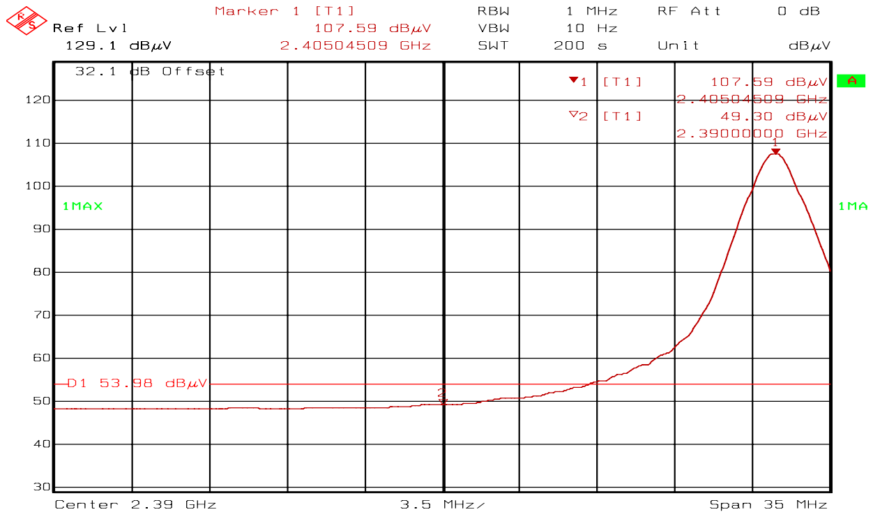
Figure 26 Low Channel Video Average
