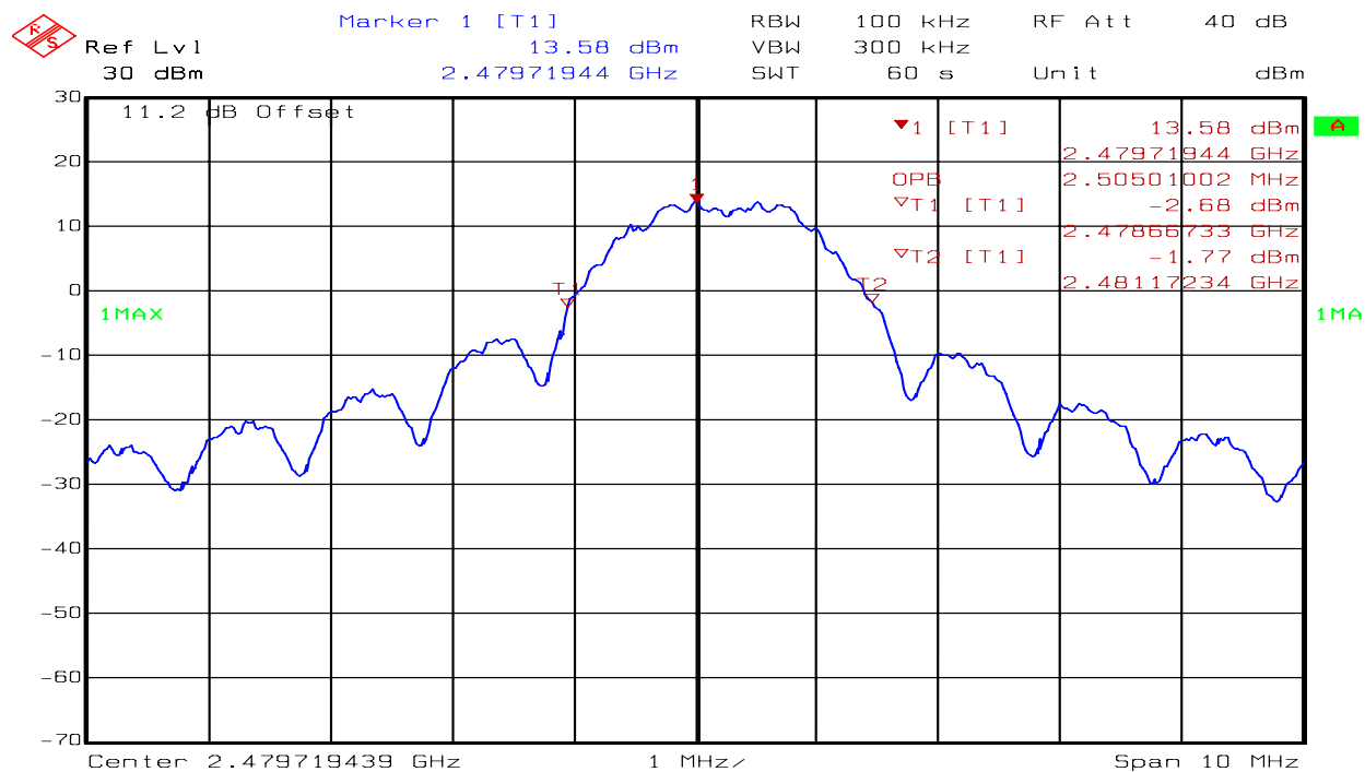
Figure 10 Occupied Bandwidth High Channel
