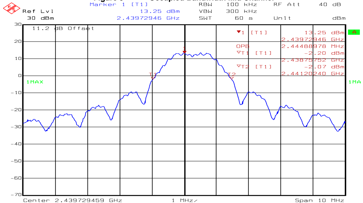
Figure 9 Occupied Bandwidth Mid Channel
