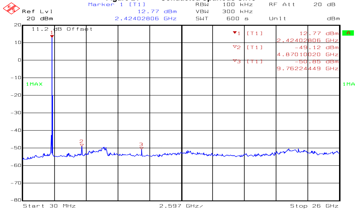
Figure 21 Conducted Spurious Ch18
