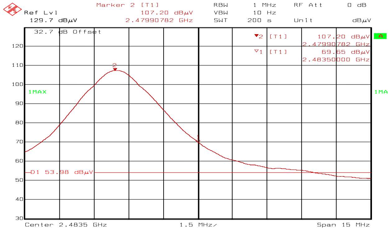
Figure 29 High Channel Video Average
