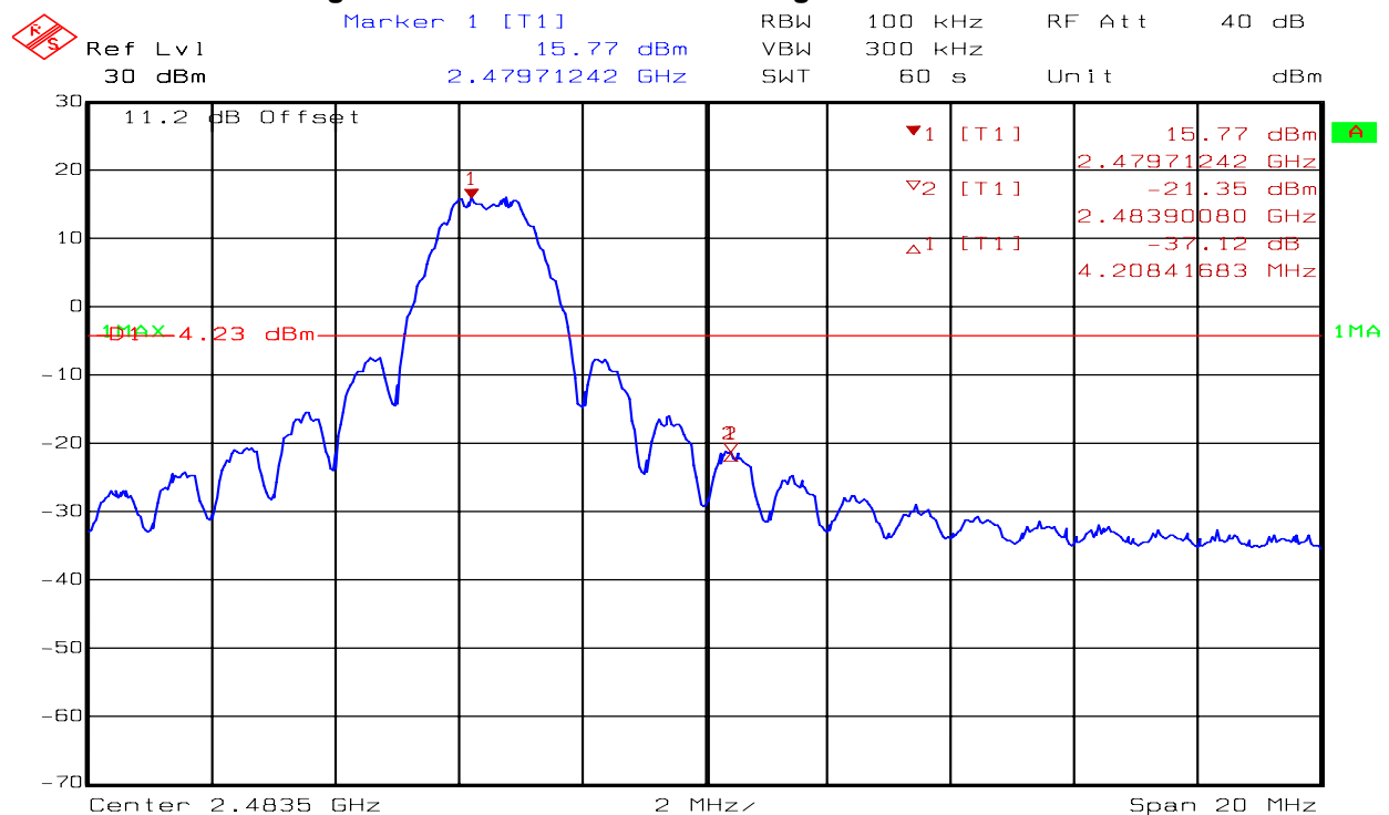
Figure 24 Conducted Band edge Measurement Ch26
