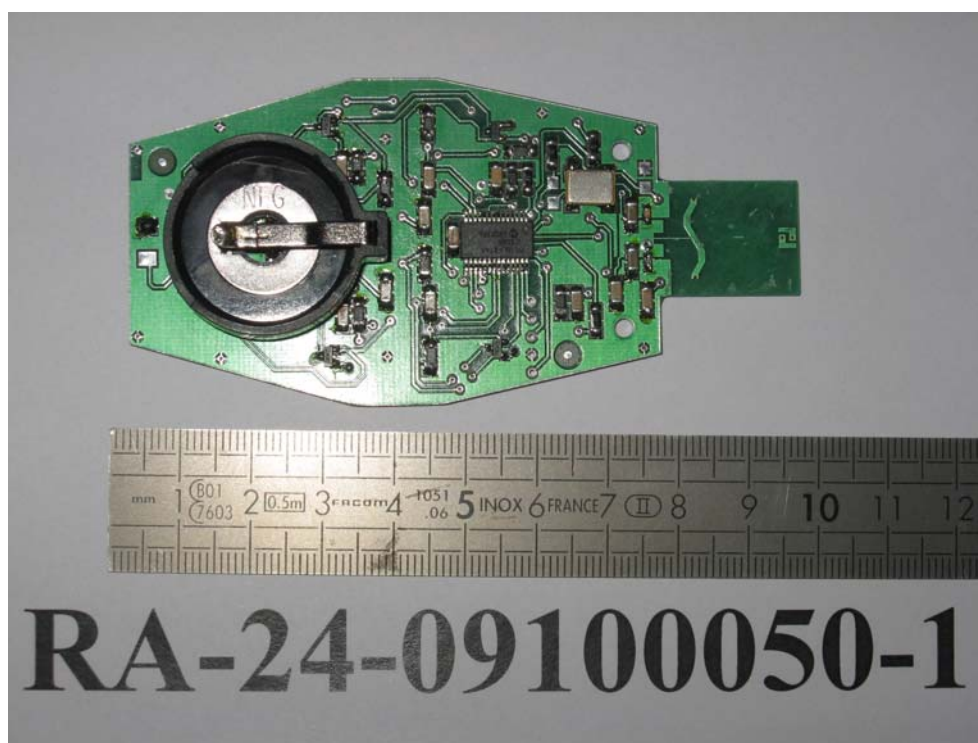
Printed circuit board transmitter: face 1
