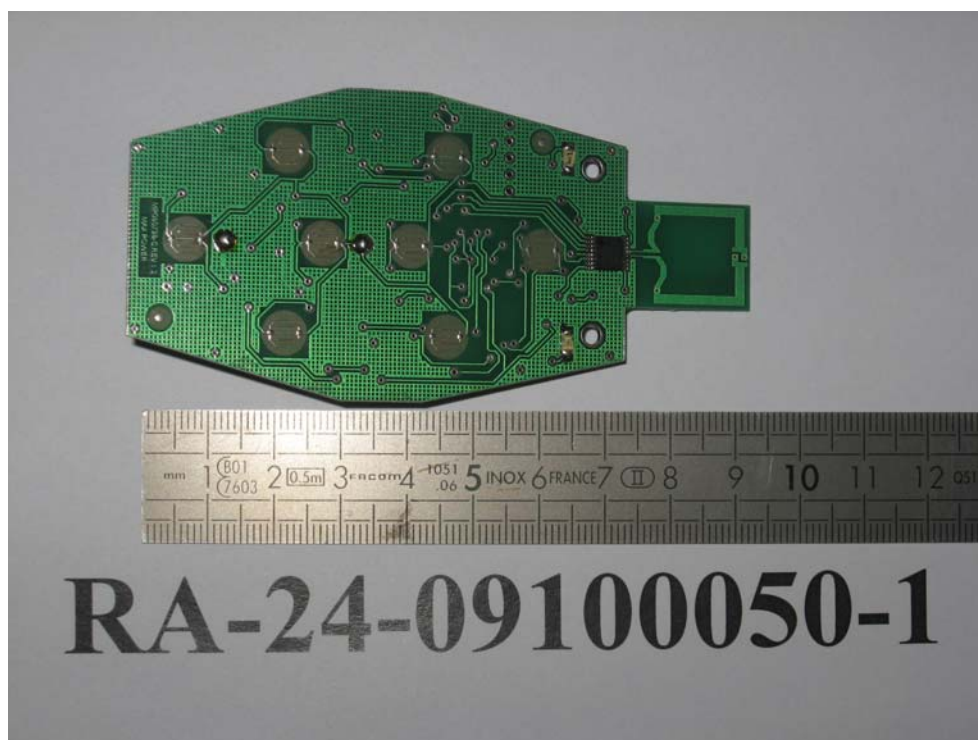
Printed circuit board transmitter: face 2
