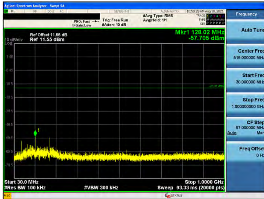
Conducted Spurious Emission (CH 11)
