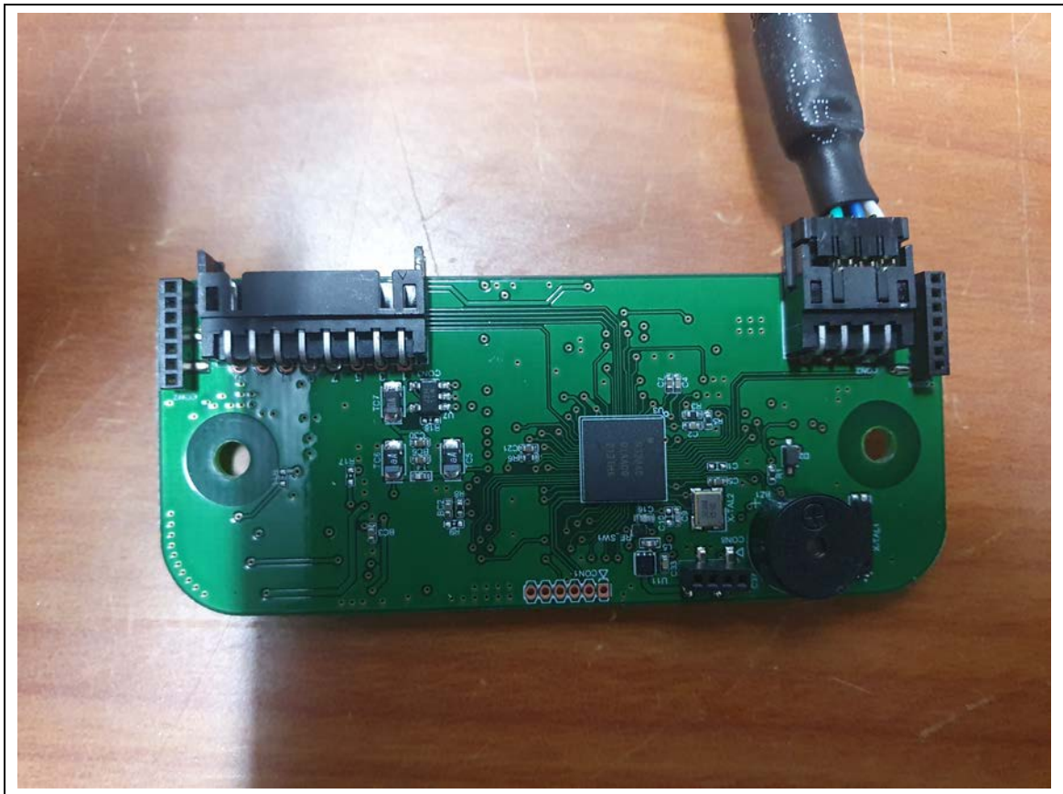
MainBoard-Rear
