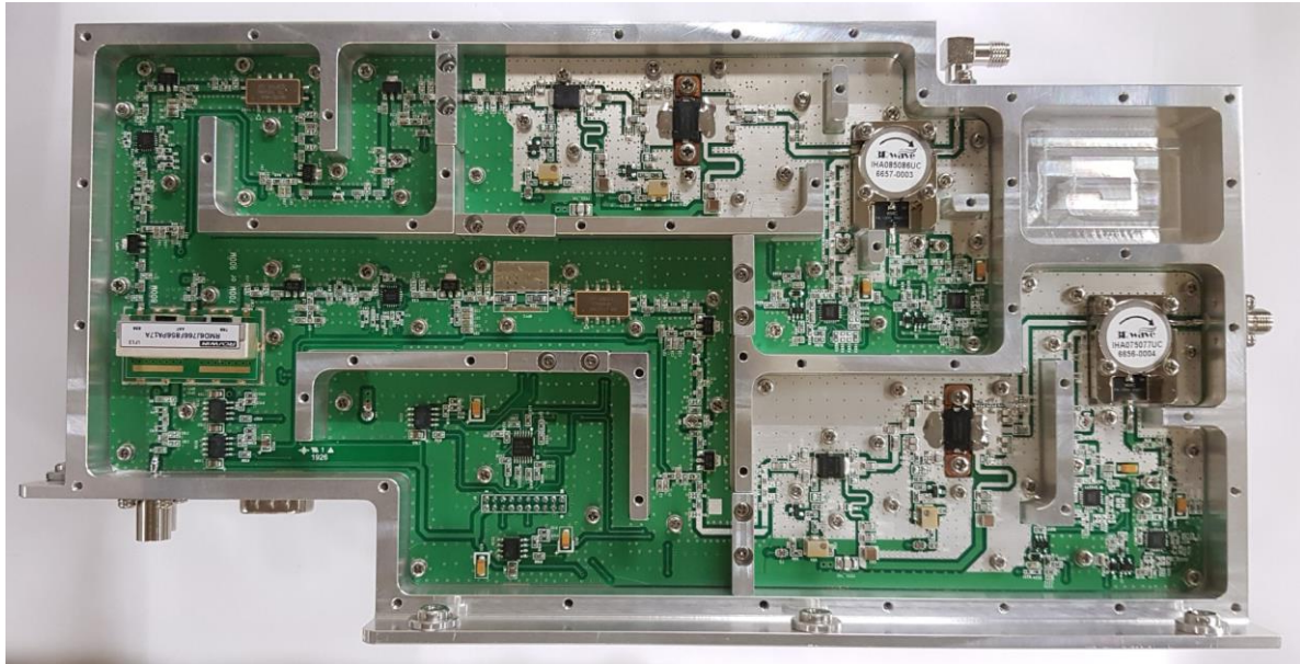
TX Inside
