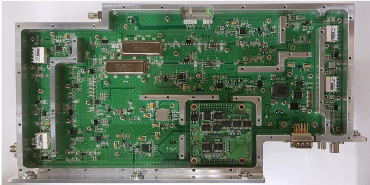
RX Inside
