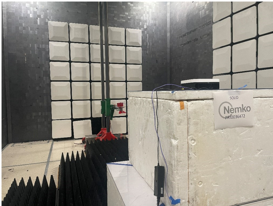
Figure 4 - Radiated emissions above 1 GHz (1 – 18 GHz), rear view.
