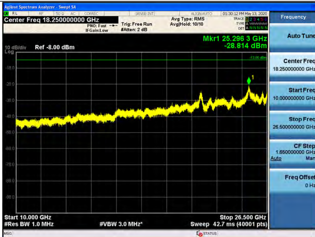
Spurious / AWS / Downlink / CDMA / Low / 10 GHz ~ 26.5 GHz
