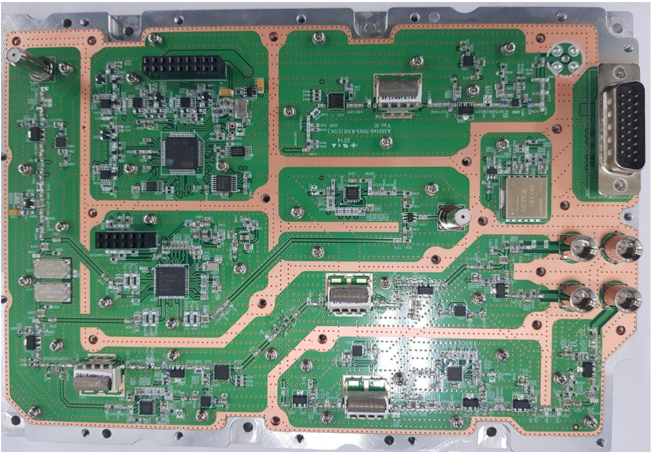
[UDCU inside]
