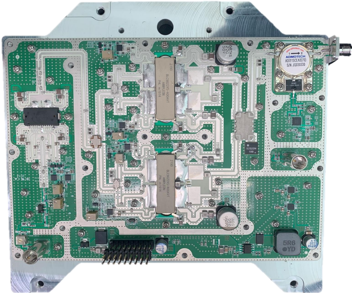
[PAU inside]
