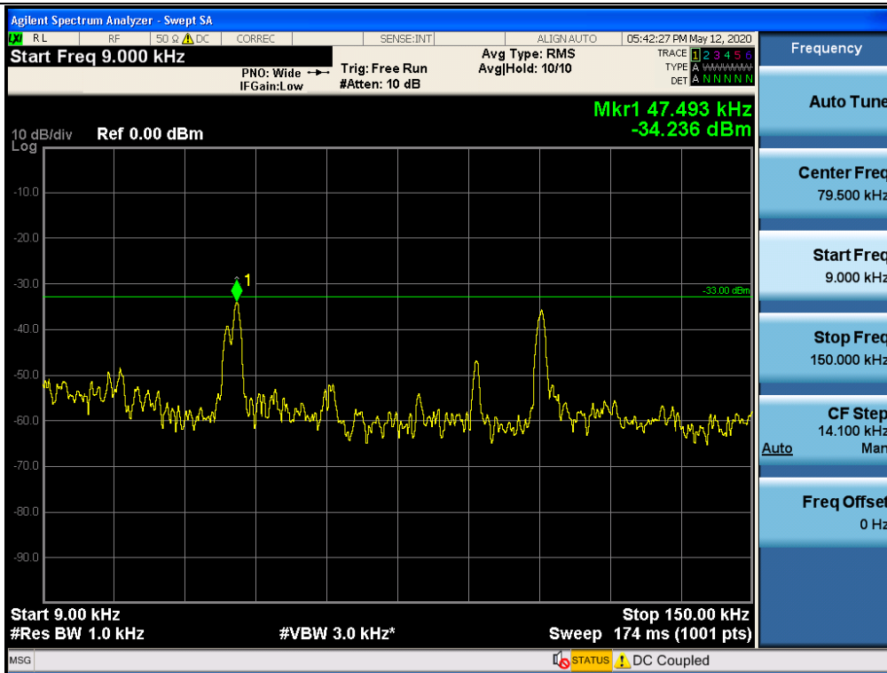
Spurious / Cellular / Downlink / LTE 10 MHz / Middle / 9 kHz ~ 150 kHz
