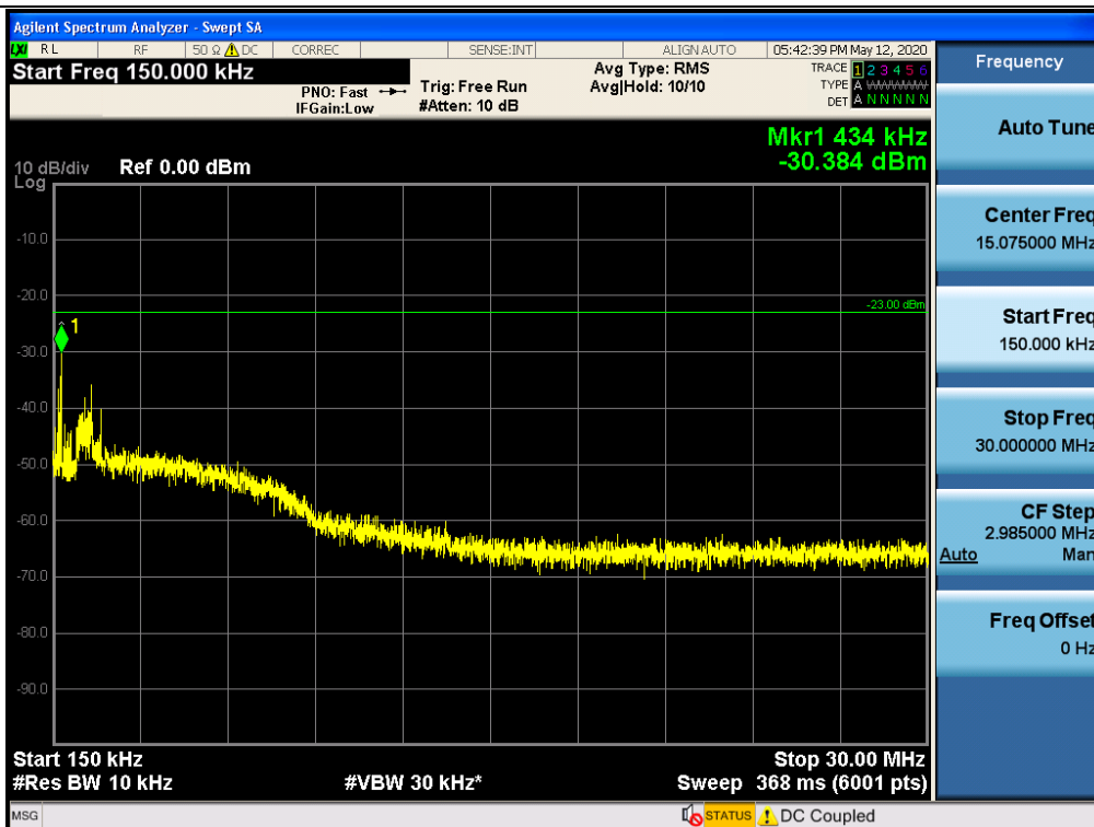
Spurious / Cellular / Downlink / LTE 10 MHz / Middle / 150 kHz ~ 30 MHz
