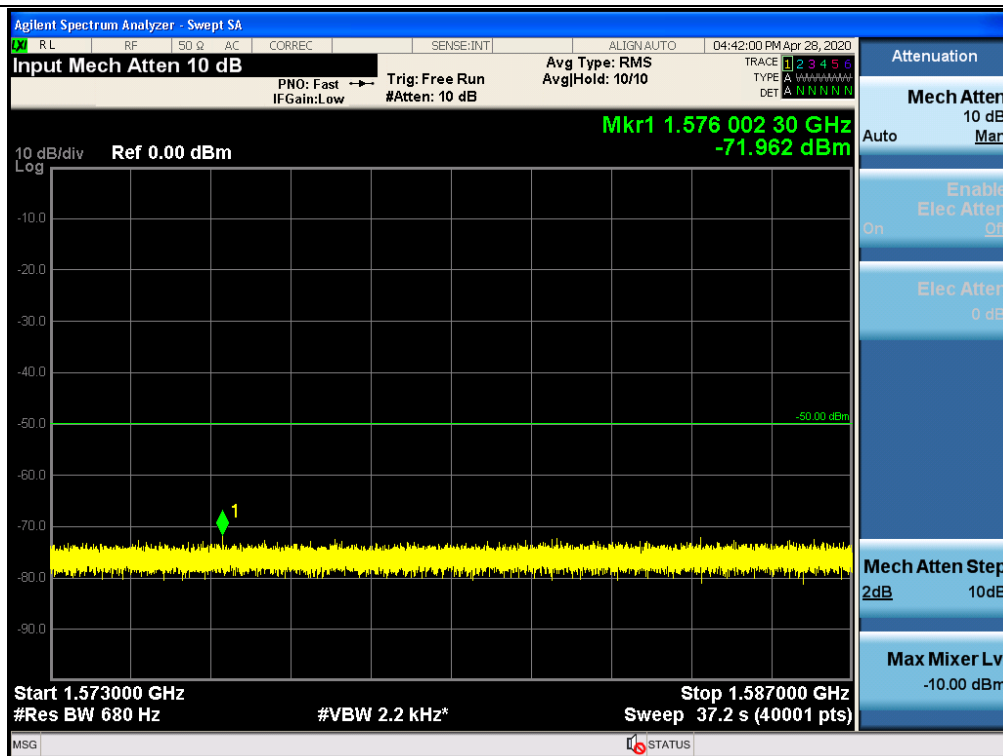
Spurious / FirstNet / Downlink/ LTE 10 MHz / Middle / Additional Band 5
