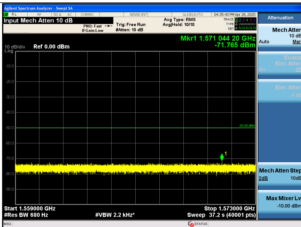
Spurious / FirstNet / Downlink/ LTE 10 MHz / Middle / Additional Band 4
