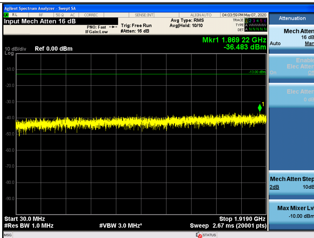
Spurious / PCS / Downlink / LTE 10 MHz / Low / 30 MHz ~ Low Edge-10
