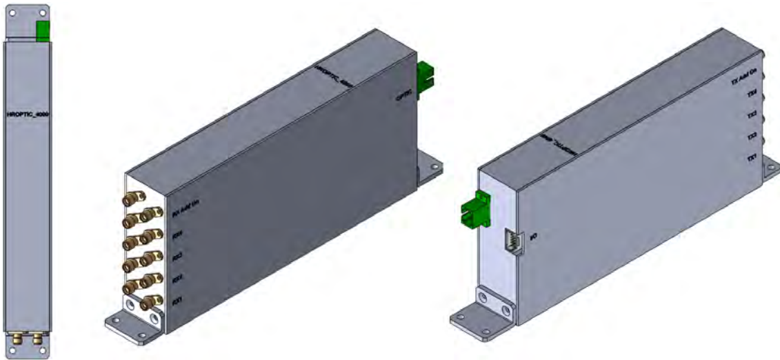
Figure 9. ROPTIC External Appearance
