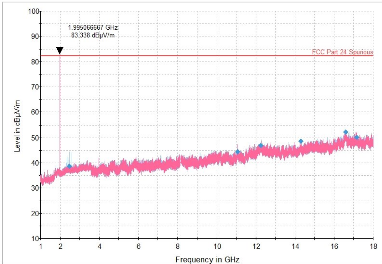
Figure 8.6-8: Radiated emissions spectral plot (1 GHz - 18 GHz) – 1995 MHz
