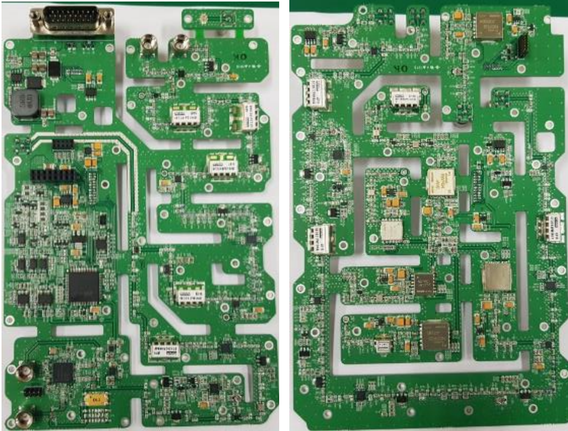
[UDC PBA Top]
