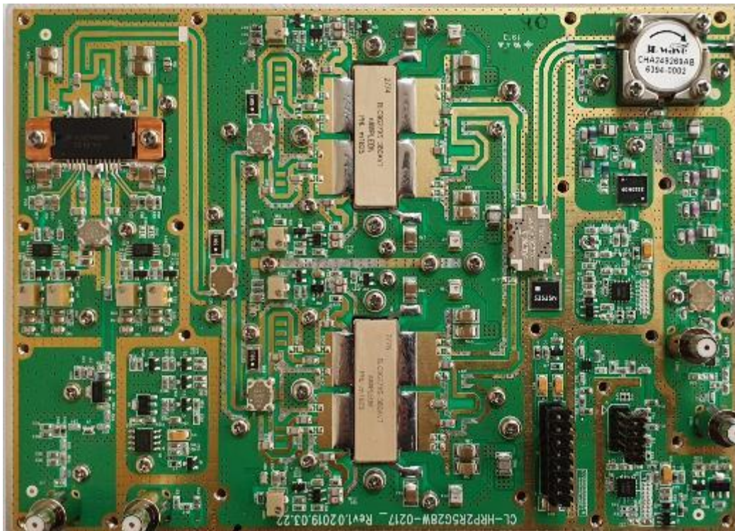
[Main/APD PBA Top]
