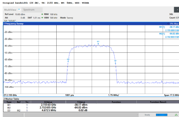
Figure 8.3-7: Occupied bandwidth / Input Versus Output Comparison results, broadband signal, 0.5 dB below AGC threshold, input and output signal respectively
