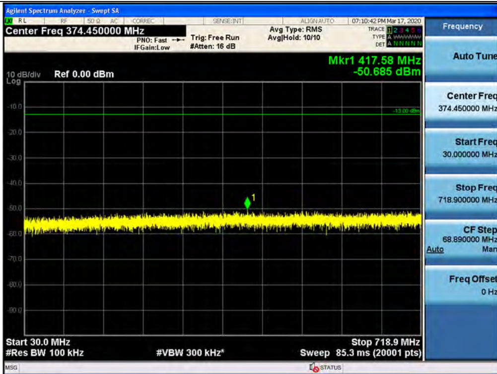
Spurious / Lower 700 MHz / Downlink / LTE 5 MHz / Middle / 30 MHz ~ Low Edge - 1.1 MHz
