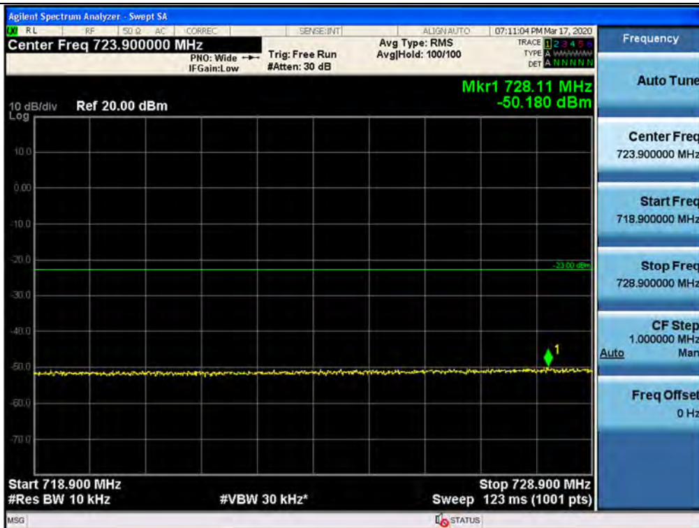
Spurious / Lower 700 MHz / Downlink / LTE 5 MHz / Middle / Low Edge - 1.1 MHz ~ Low Edge - 100 kHz
