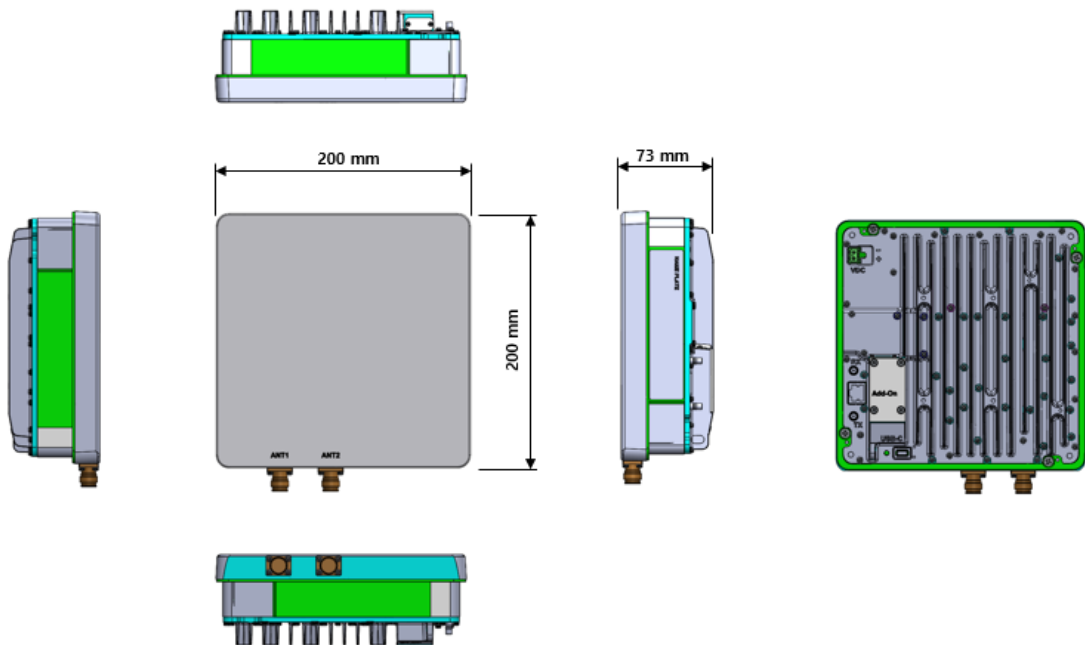
Figure 3. Dimension used to install eROU (external)
