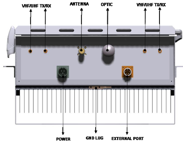
Figure 4.31 – ROU Bottom Look
