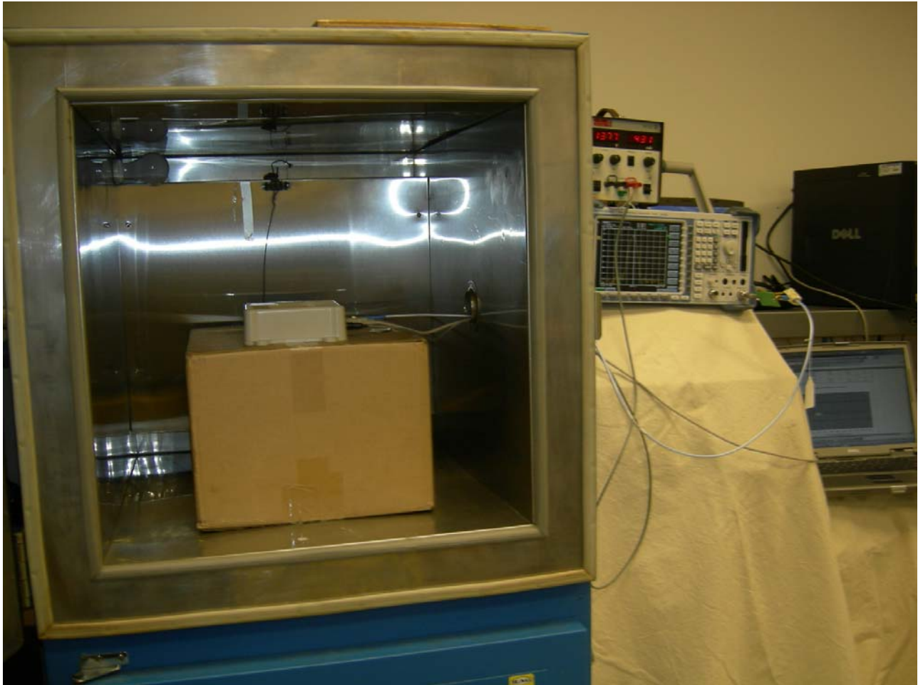
Figure 2: Frequency Stability
