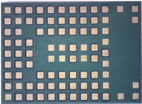
Figure 7: Bottom view of MAYA-W161-00B, MAYA-W166-00B and MAYA-W166-01B
