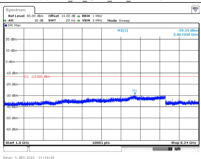
821.5 MHz_5M_QPSK_1RB_Above 1GHz
