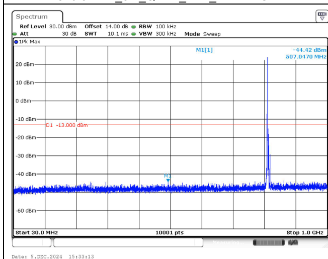
816.5 MHz_5M_QPSK_1RB_Below 1GHz
