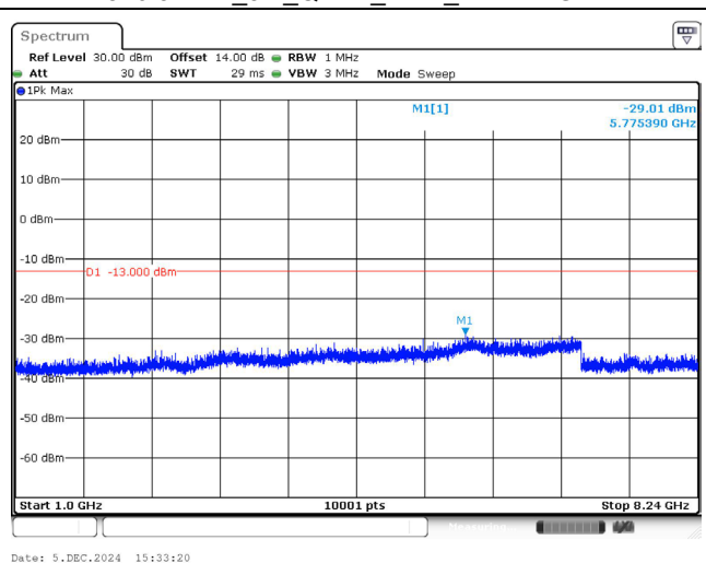
816.5 MHz_5M_QPSK_1RB_Above 1GHz
