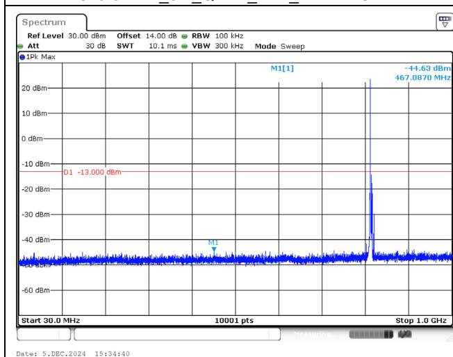
821.5 MHz_5M_QPSK_1RB_Below 1GHz
