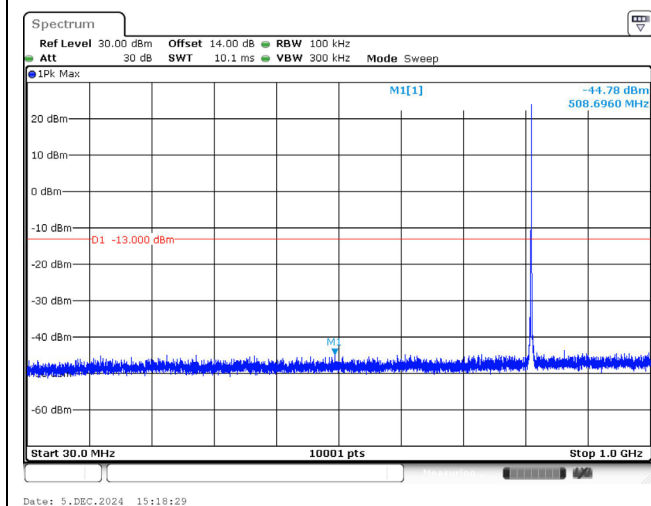
814.7 MHz_1.4M_QPSK_1RB_Below 1GHz
