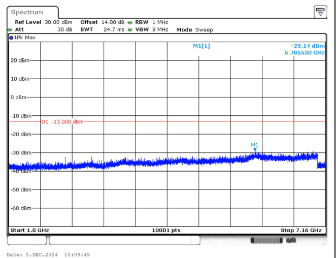
707.5 MHz_10M_QPSK_1RB_Above 1GHz
