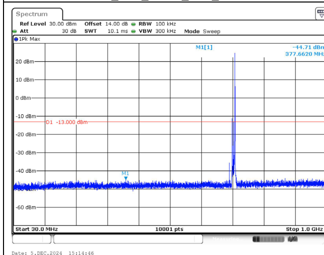
711.0 MHz_10M_QPSK_1RB_Below 1GHz
