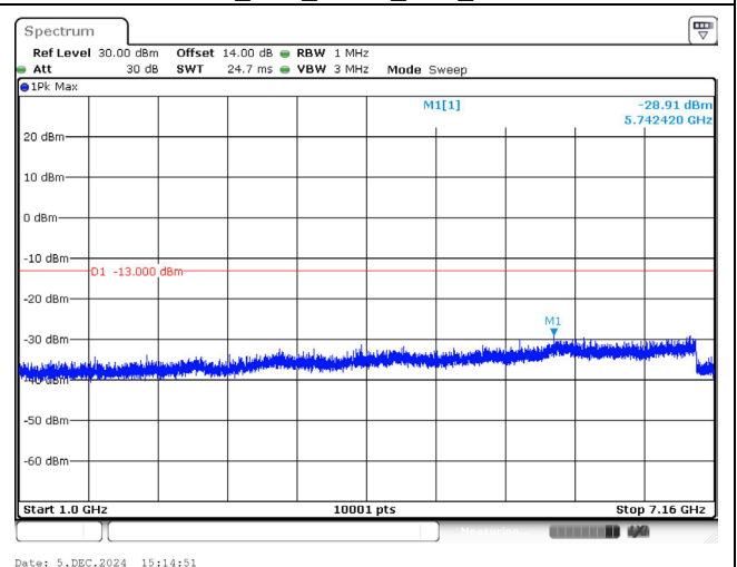
711.0 MHz_10M_QPSK_1RB_Above 1GHz
