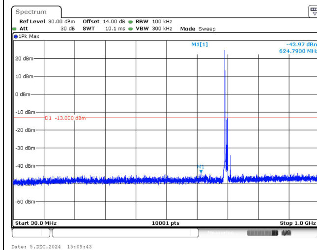
707.5 MHz_10M_QPSK_1RB_Below 1GHz
