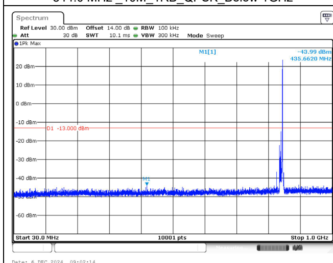
844.0 MHz _10M_1RB_QPSK_Below 1GHz
