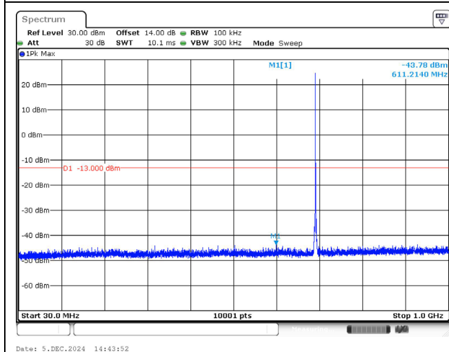
699.7 MHz_1.4M_QPSK_1RB_Below 1GHz
