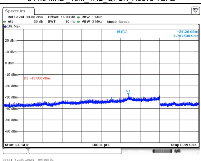
841.5 MHz _15M_1RB_QPSK_Above 1GHz
