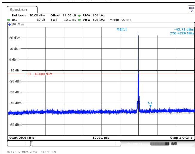
713.5 MHz_5M_QPSK_1RB_Below 1GHz
