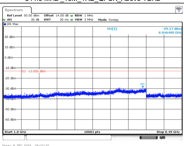
844.0 MHz _10M_1RB_QPSK_Above 1GHz
