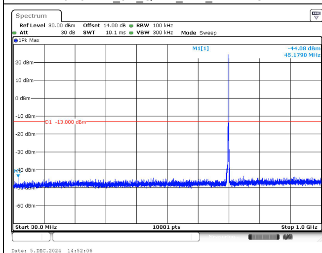
707.5 MHz_3M_QPSK_1RB_Below 1GHz
