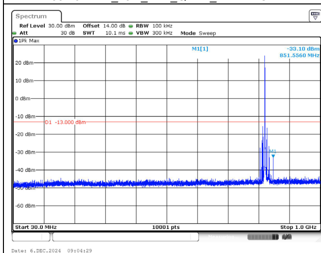
836.5 MHz _15M_1RB_QPSK_Below 1GHz
