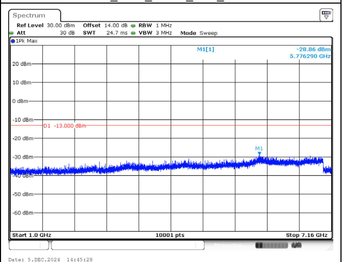
715.3 MHz_1.4M_QPSK_1RB_Above 1GHz
