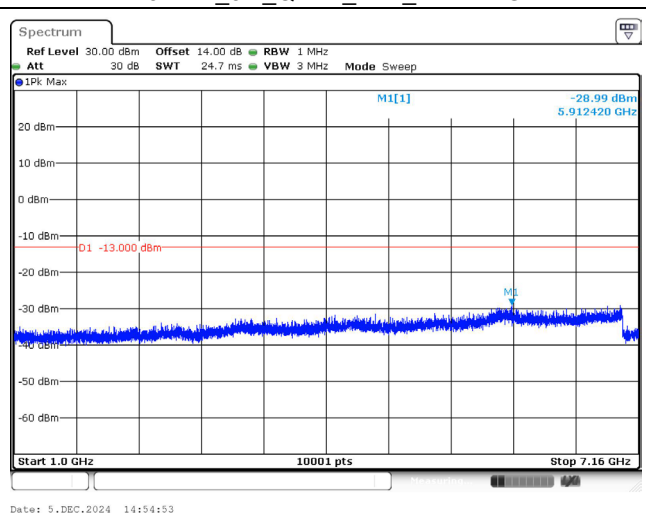
714.5 MHz_3M_QPSK_1RB_Above 1GHz
