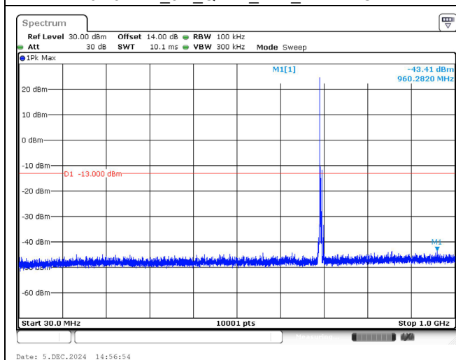
707.5 MHz_5M_QPSK_1RB_Below 1GHz
