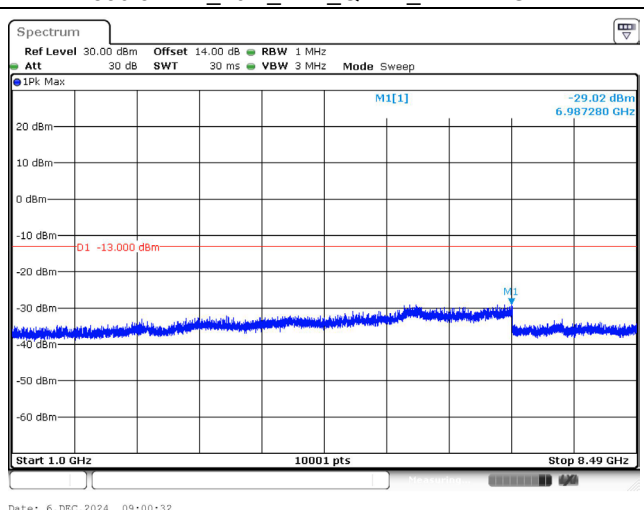
836.5 MHz _10M_1RB_QPSK_Above 1GHz
