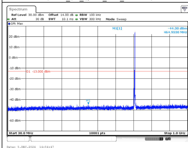
714.5 MHz_3M_QPSK_1RB_Below 1GHz
