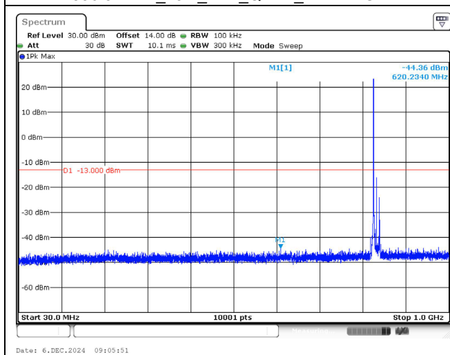
841.5 MHz _15M_1RB_QPSK_Below 1GHz
