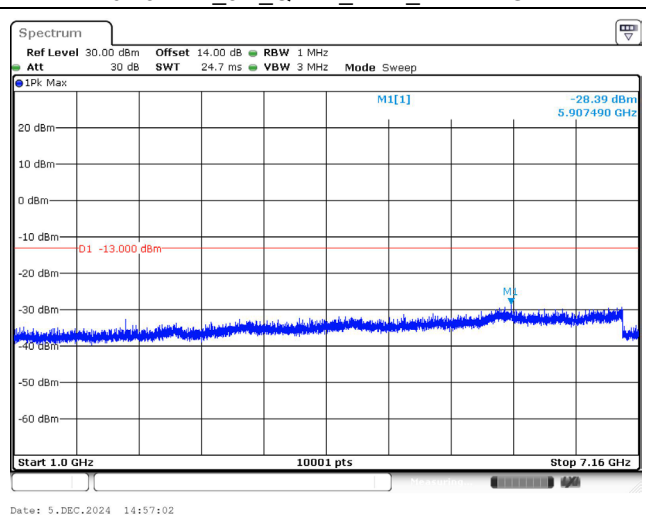
707.5 MHz_5M_QPSK_1RB_Above 1GHz
