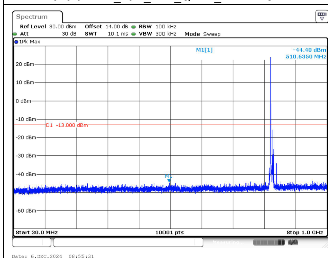
829.0 MHz _10M_1RB_QPSK_Below 1GHz
