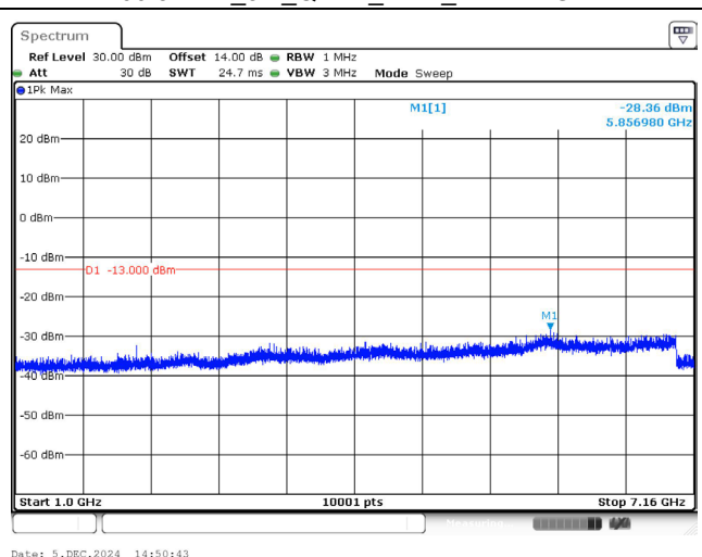
700.5 MHz_3M_QPSK_1RB_Above 1GHz
