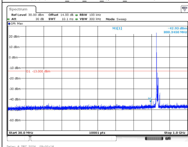
836.5 MHz _10M_1RB_QPSK_Below 1GHz
