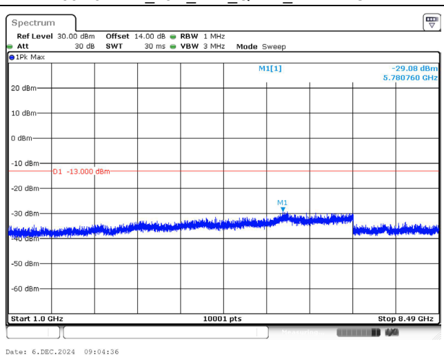
836.5 MHz _15M_1RB_QPSK_Above 1GHz
