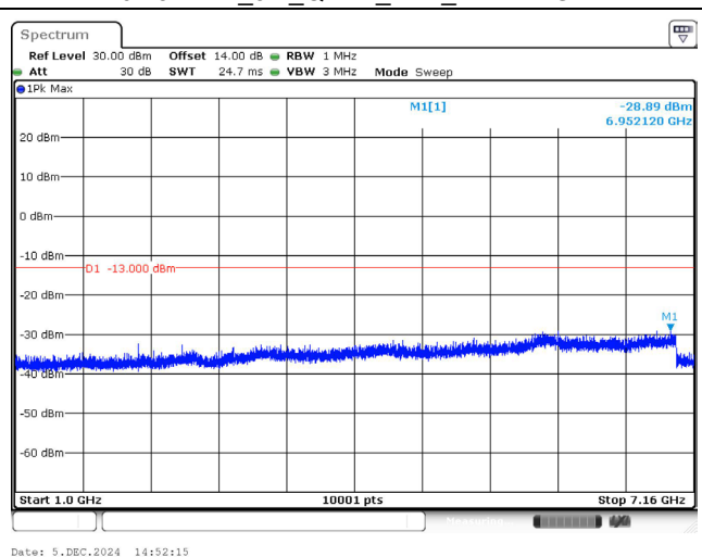
707.5 MHz_3M_QPSK_1RB_Above 1GHz
