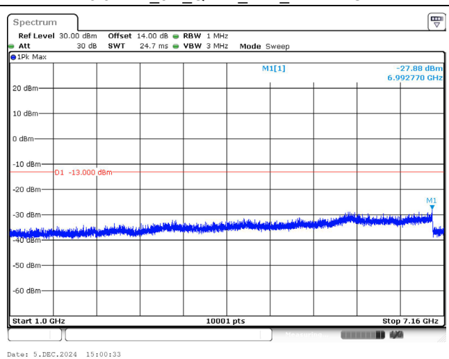
713.5 MHz_5M_QPSK_1RB_Above 1GHz
