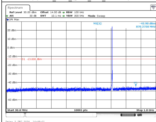
715.3 MHz_1.4M_QPSK_1RB_Below 1GHz
