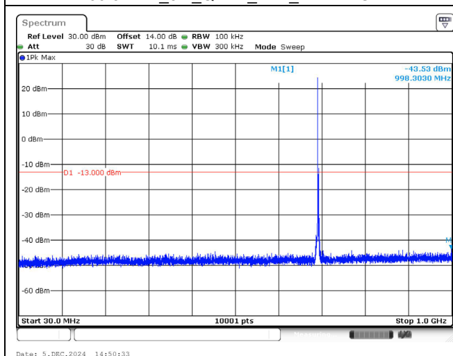
700.5 MHz_3M_QPSK_1RB_Below 1GHz
