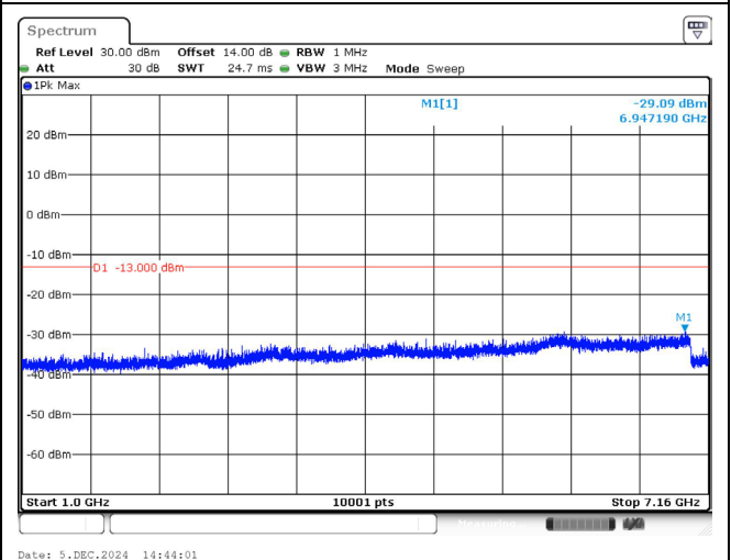
699.7 MHz_1.4M_QPSK_1RB_Above 1GHz
