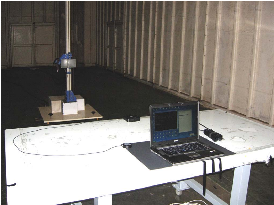
Back View of Radiated Test (Horn) – Mode 3~Mode 4
