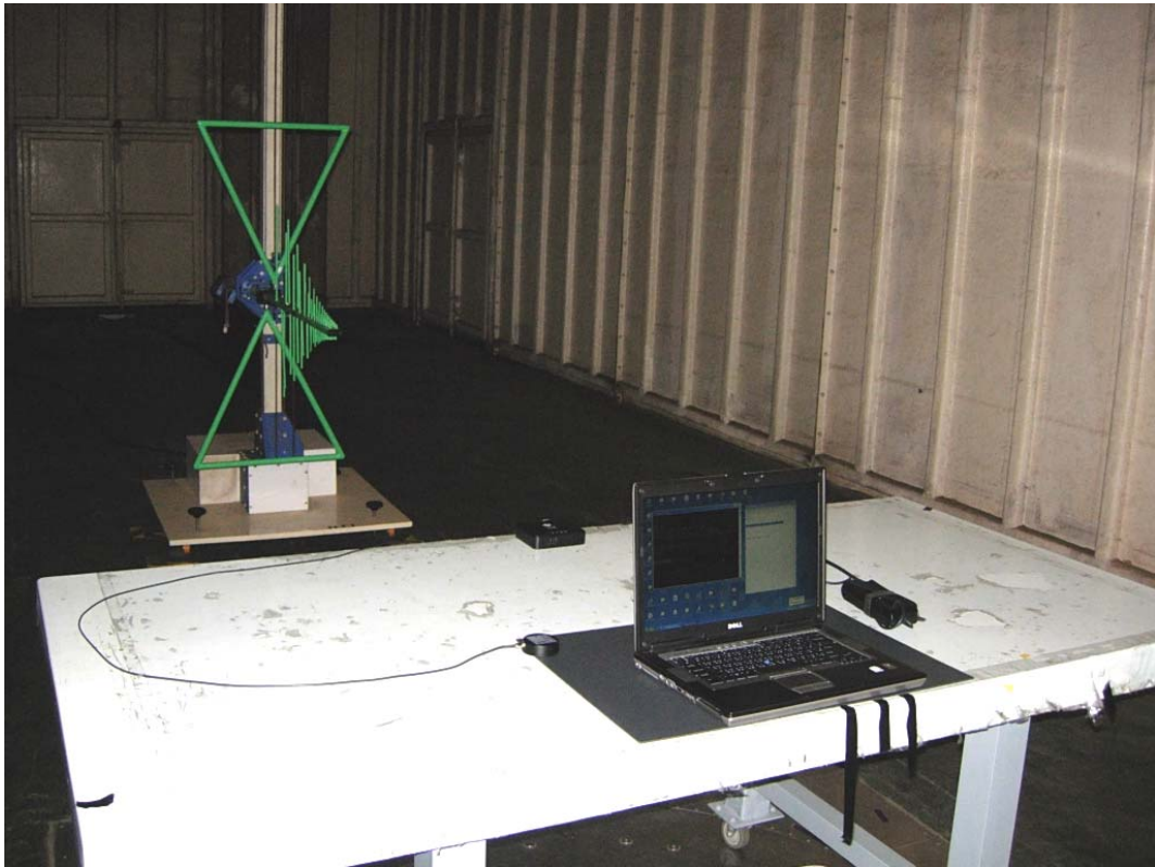
Back View of Radiated Test – Mode 3~Mode 4
