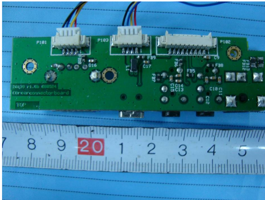
EUT – Rear Connect Board Bottom View
