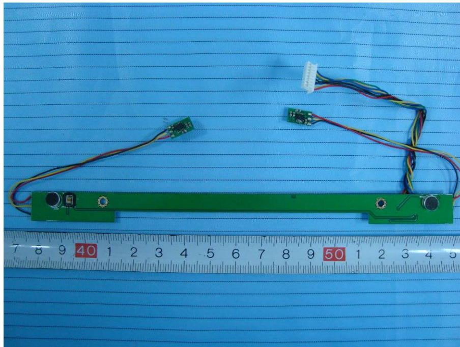
EUT – Microphone Light LED Board Bottom View
