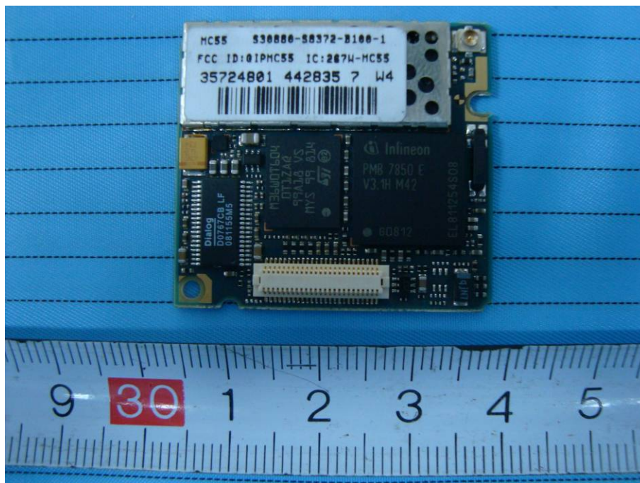
EUT – PCS Module View
