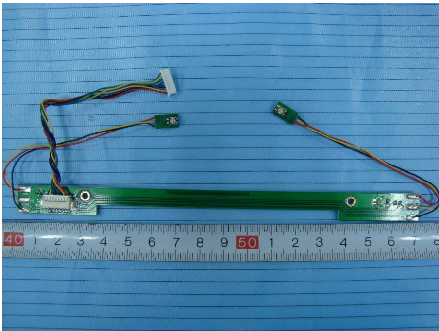
EUT – Microphone Light LED Board Top View
