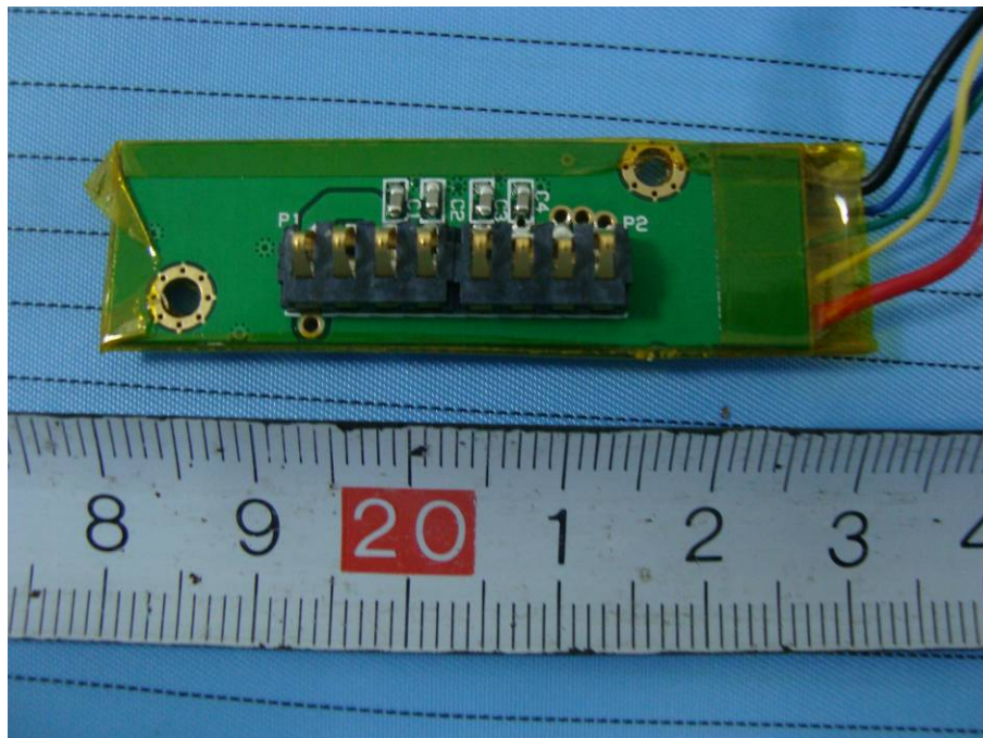
EUT – Right Battery Board Top View
