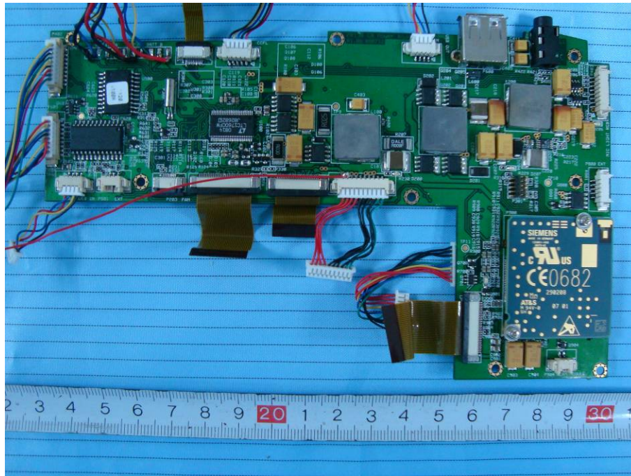
EUT – Power Board Top View 1
