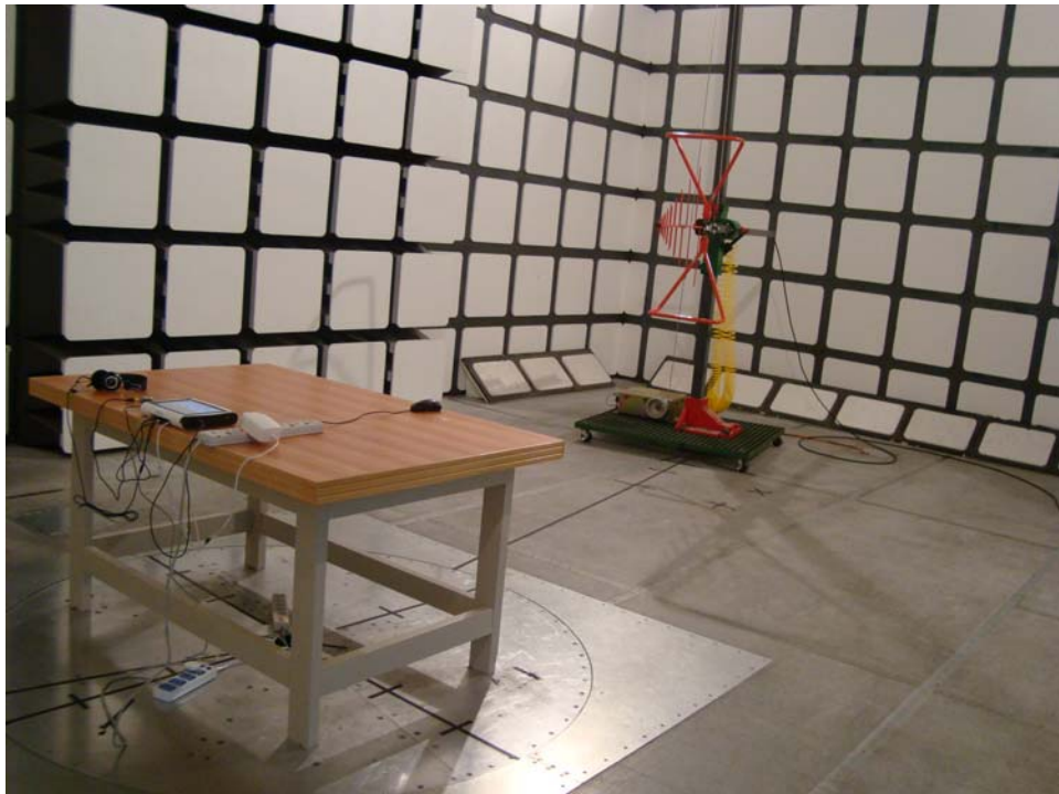
30-1000MHz: Radiated Emissions - Rear View
