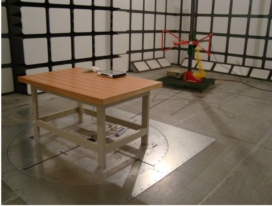
30-1000 MHz: Radiated Emissions - Rear View
