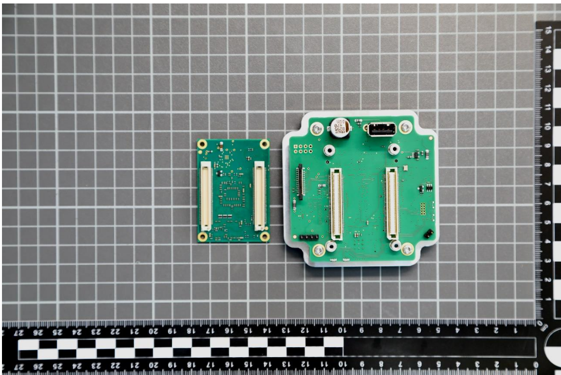
Photograph 4: EUT
