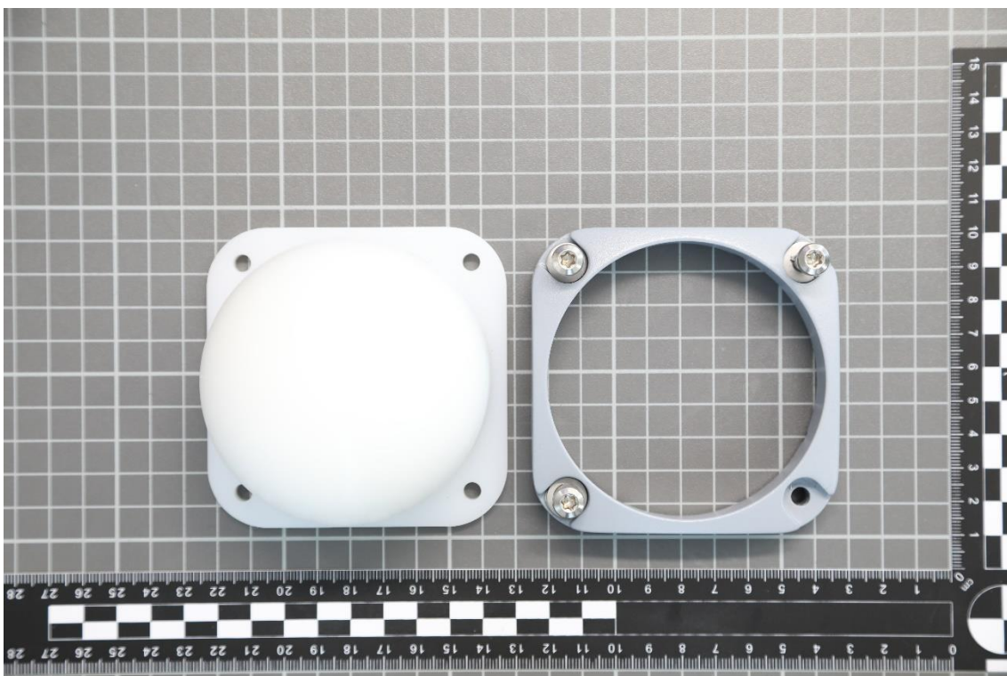
Photograph 2: EUT
