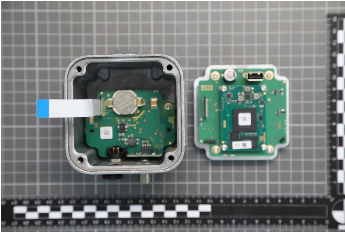
Photograph 3: EUT
