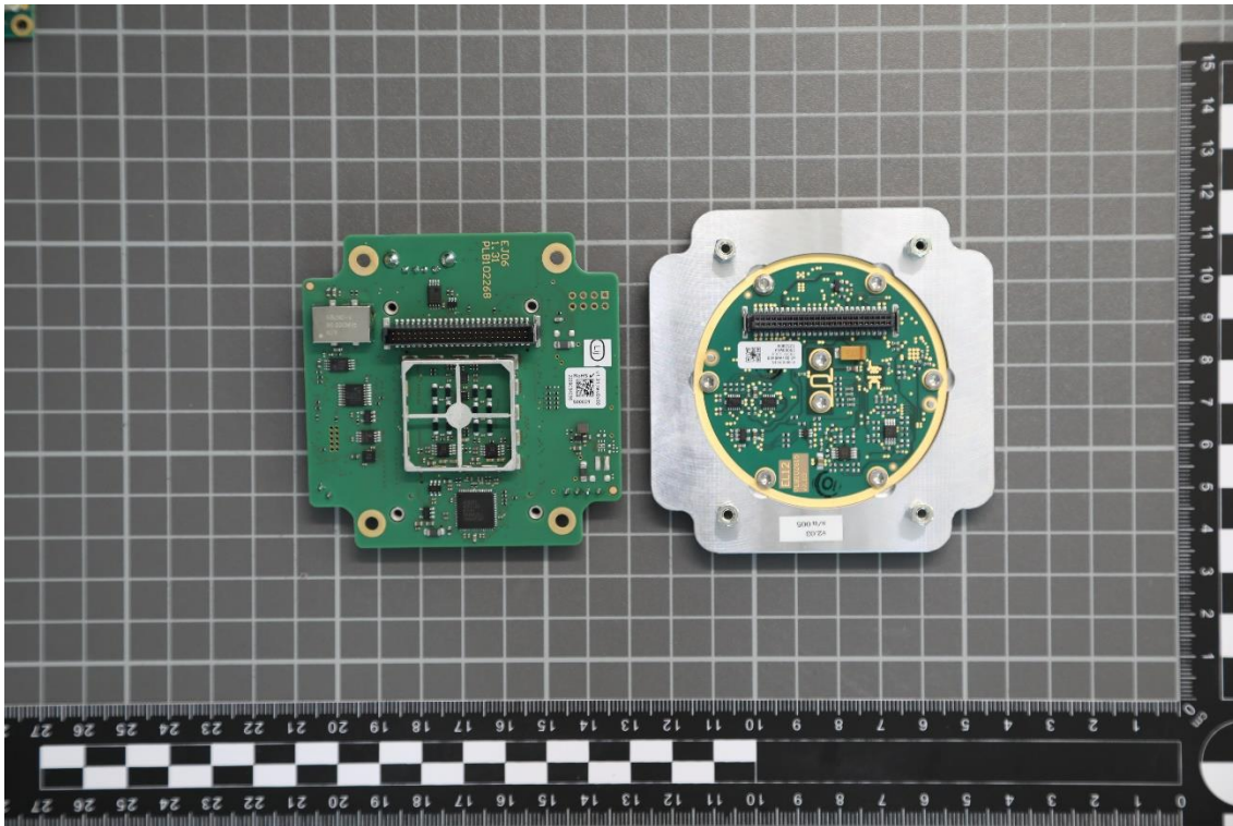
Photograph 5: EUT
