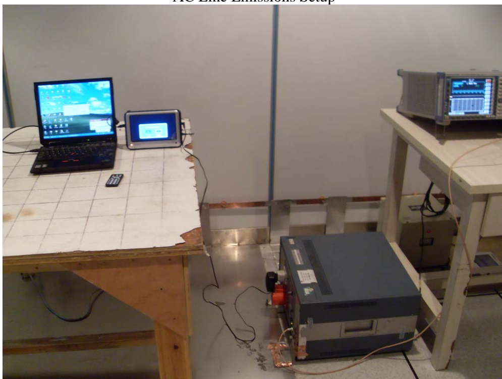
AC Line Emissions Setup
