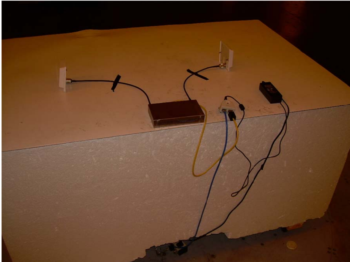
Back View Radiated Emissions Configuration – XAP-1032
