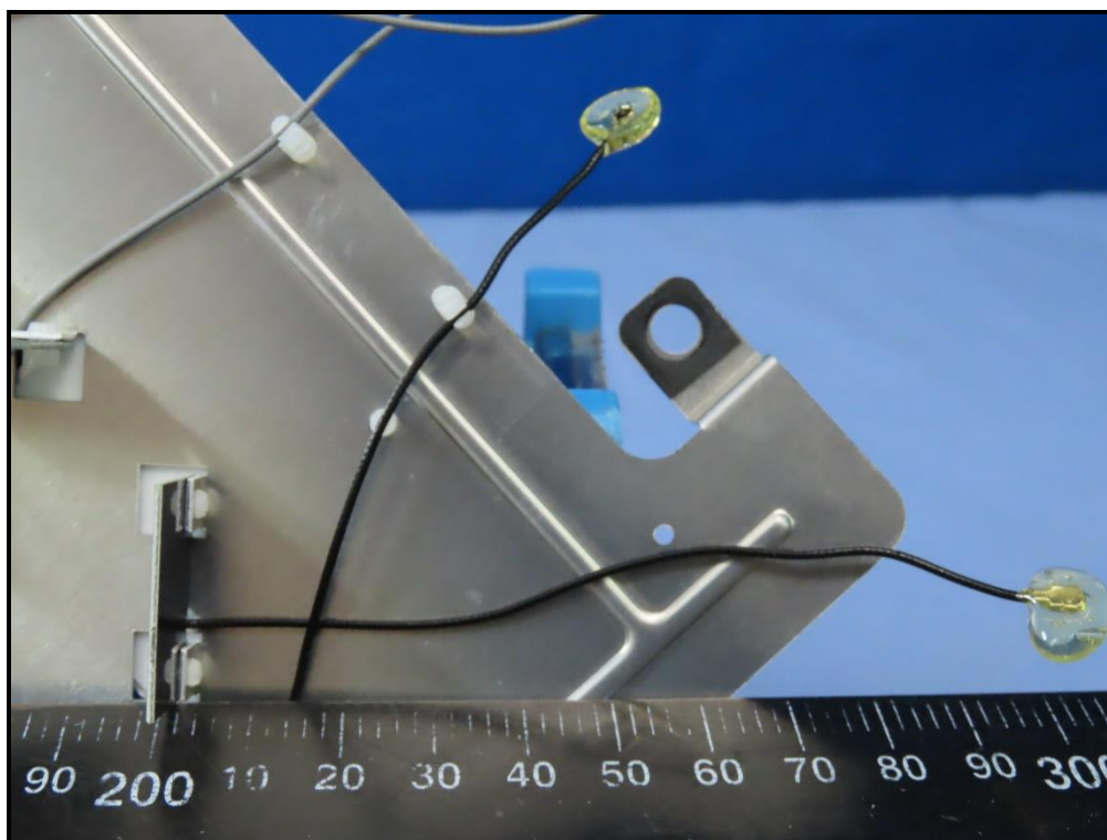
Antenna: 5G_Chain 1
