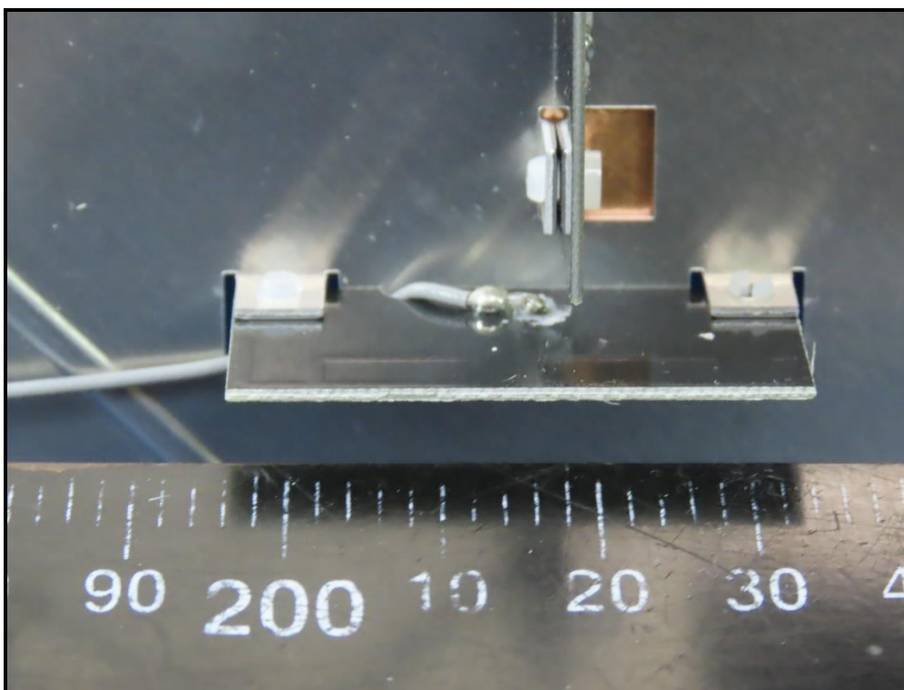
Antenna: 2G_Chain 1
