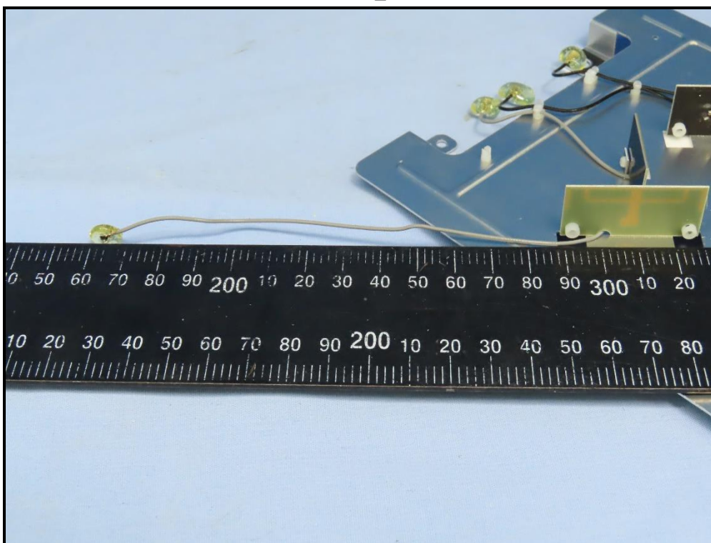
Antenna: 2G_Chain 0
