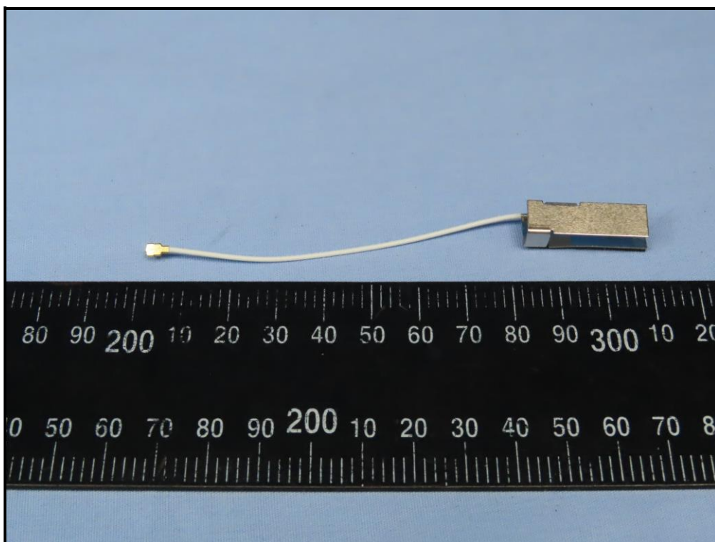
Antenna 4 (Model: 290-20495)
