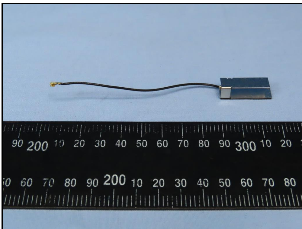
Antenna 2 (Model: 290-20493)
