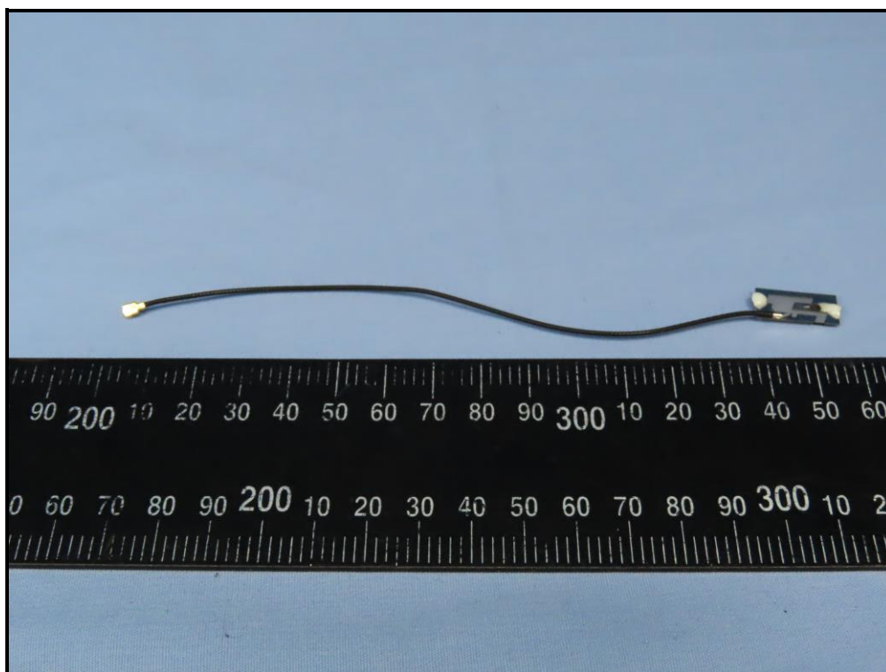
Antenna 1 (Model: 290-20492)
