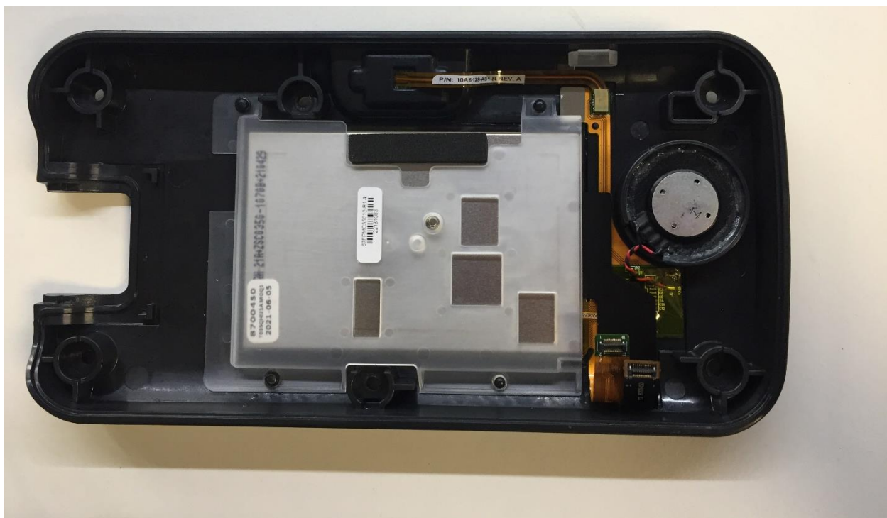
Front Cover with LCD Display – Bottom View
