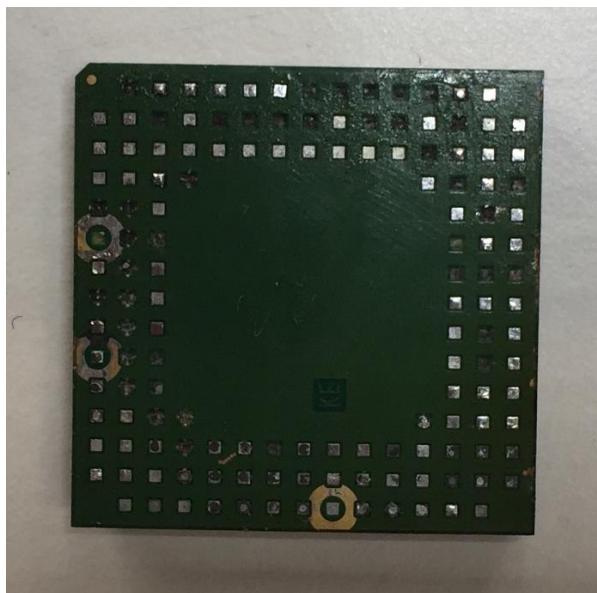
Radio Module Photo – Bottom Side View
