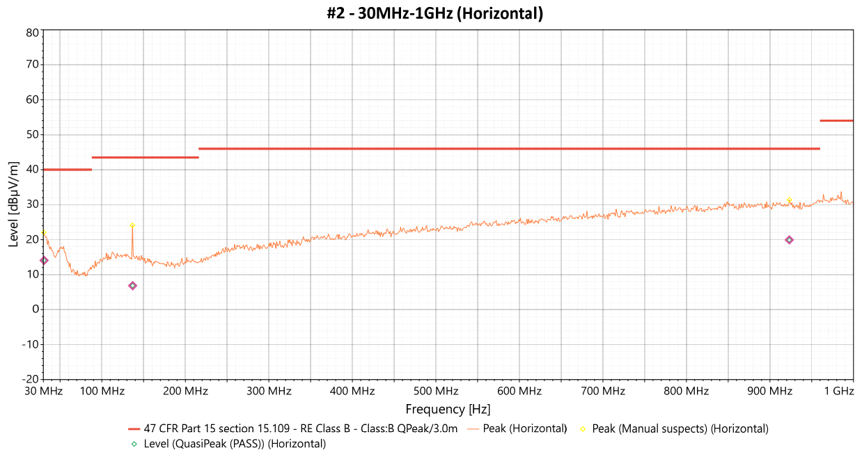
Figure 2. Radiated Emissions, Plot (Horizontal)
