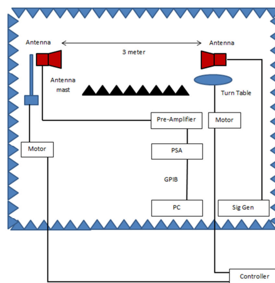
ERP / EIRP, Block Diagram, Test Setup Above 1GHz
