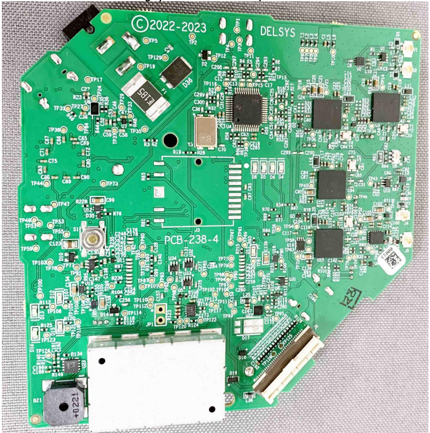
Photograph of PC Board 3: Component Side
