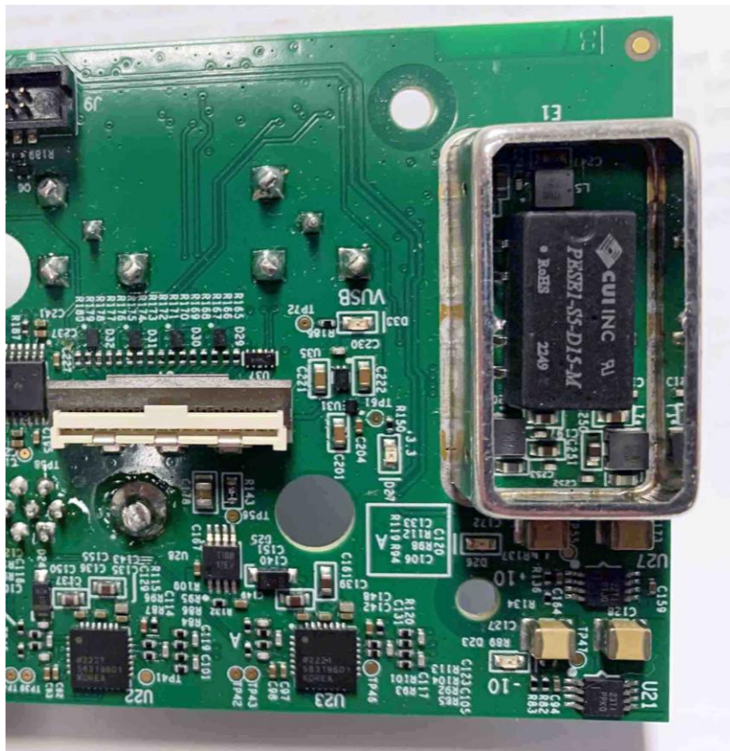
Photograph of PC Board 2; Shield removed
