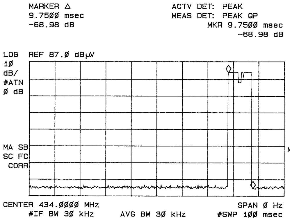
Figure six Plot of Duty Cycle in 100 mS Period
