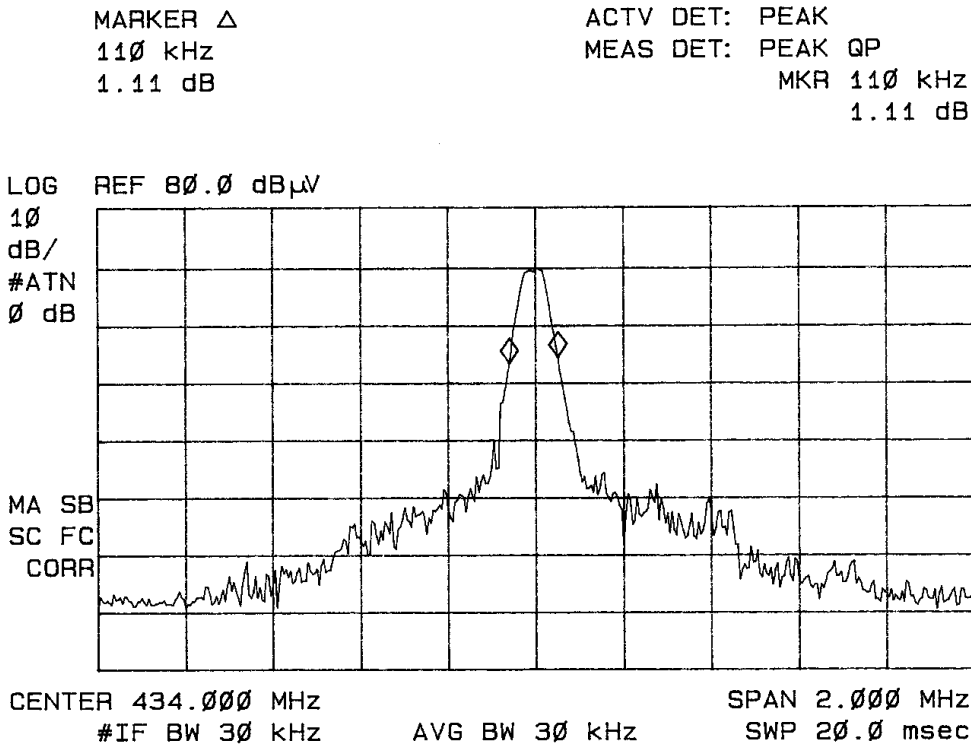
Figure five Plot of Occupied Bandwidth Emission
