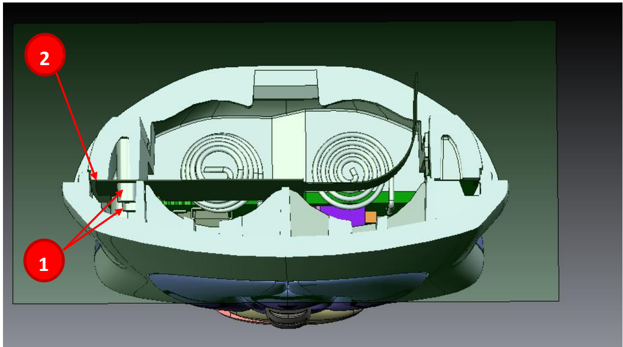
Diagram showing cross section of the remote control with a perspective from the rear to the front of the device
