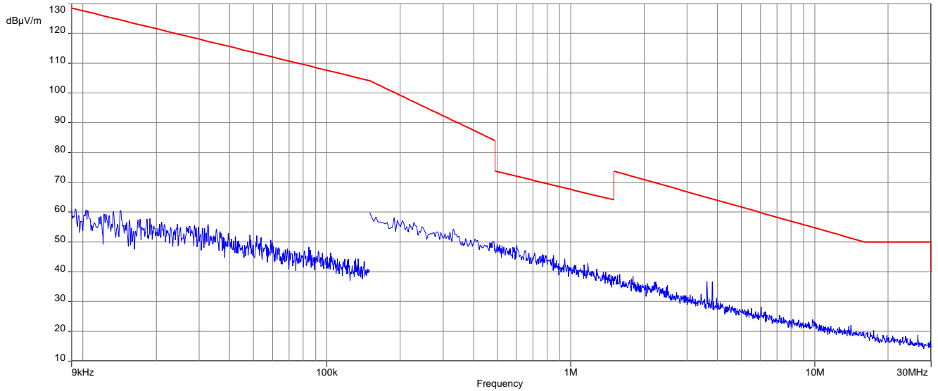
Plot 1: 9 kHz to 30 MHz, TX Mode, low channel, transmit mode
