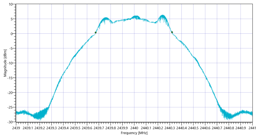
Plot_FCC Part 15.247 Maximum Peak Conducted Output Power DTS ~ BT LE 1 Msps DTS BW_11102021_165059.png
