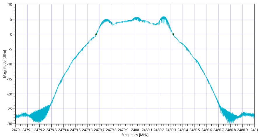
Plot_FCC Part 15.247 Bandwidth 6dB DTS ~ BT LE 1 Msps_11102021_165343.png
