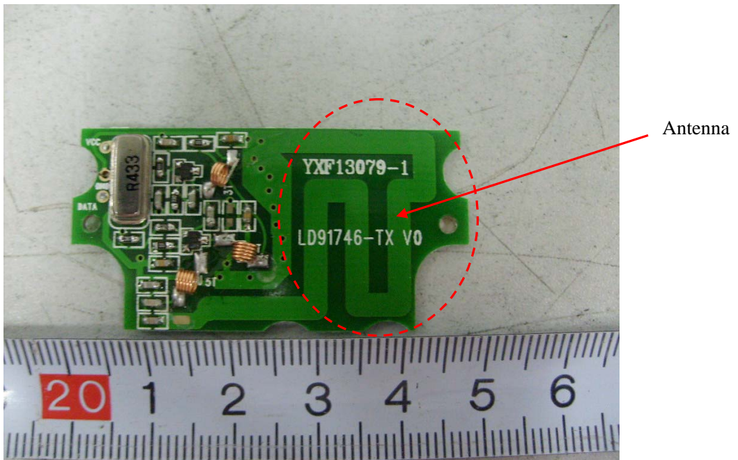
EUT- RF Board Top View
