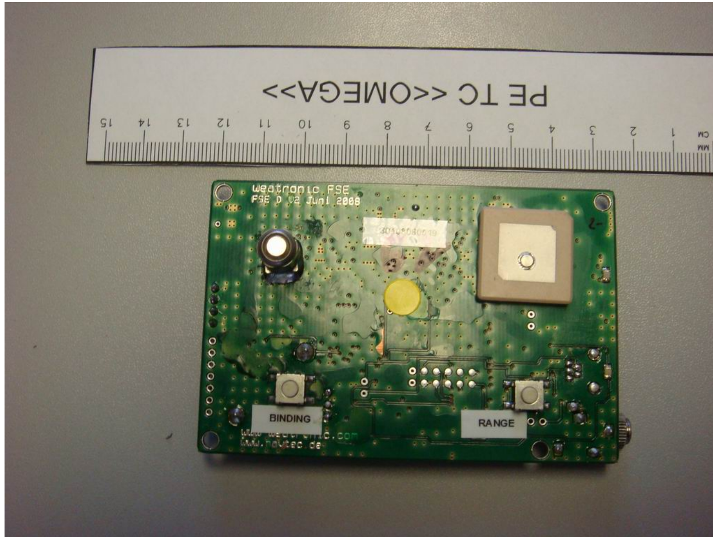
Figure 2 –Rear view.
