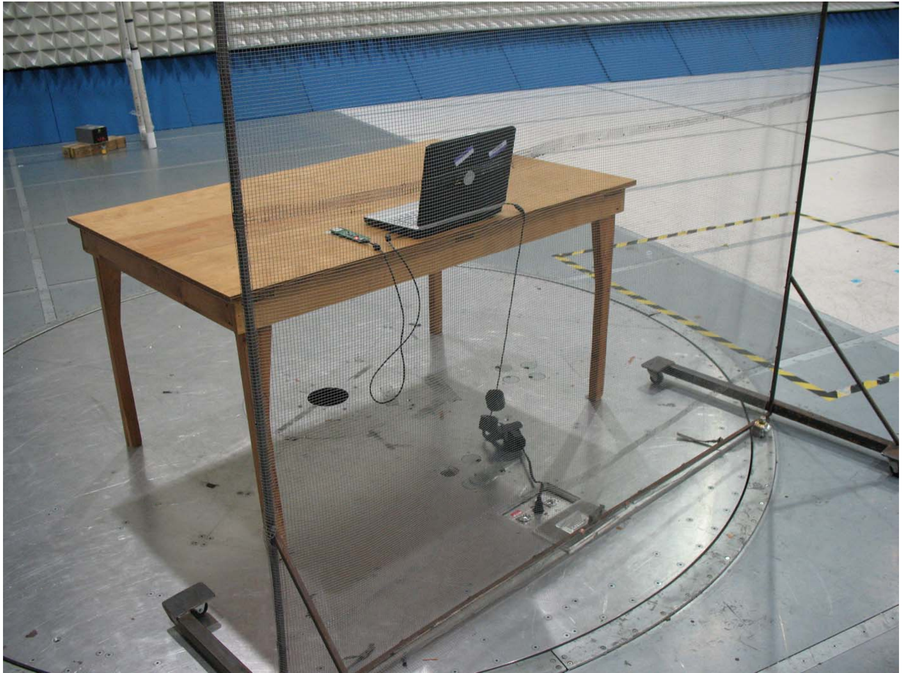
Conducted Emissions
