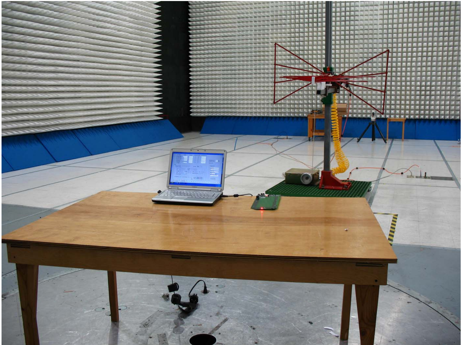
Radiated Emissions (Front)
