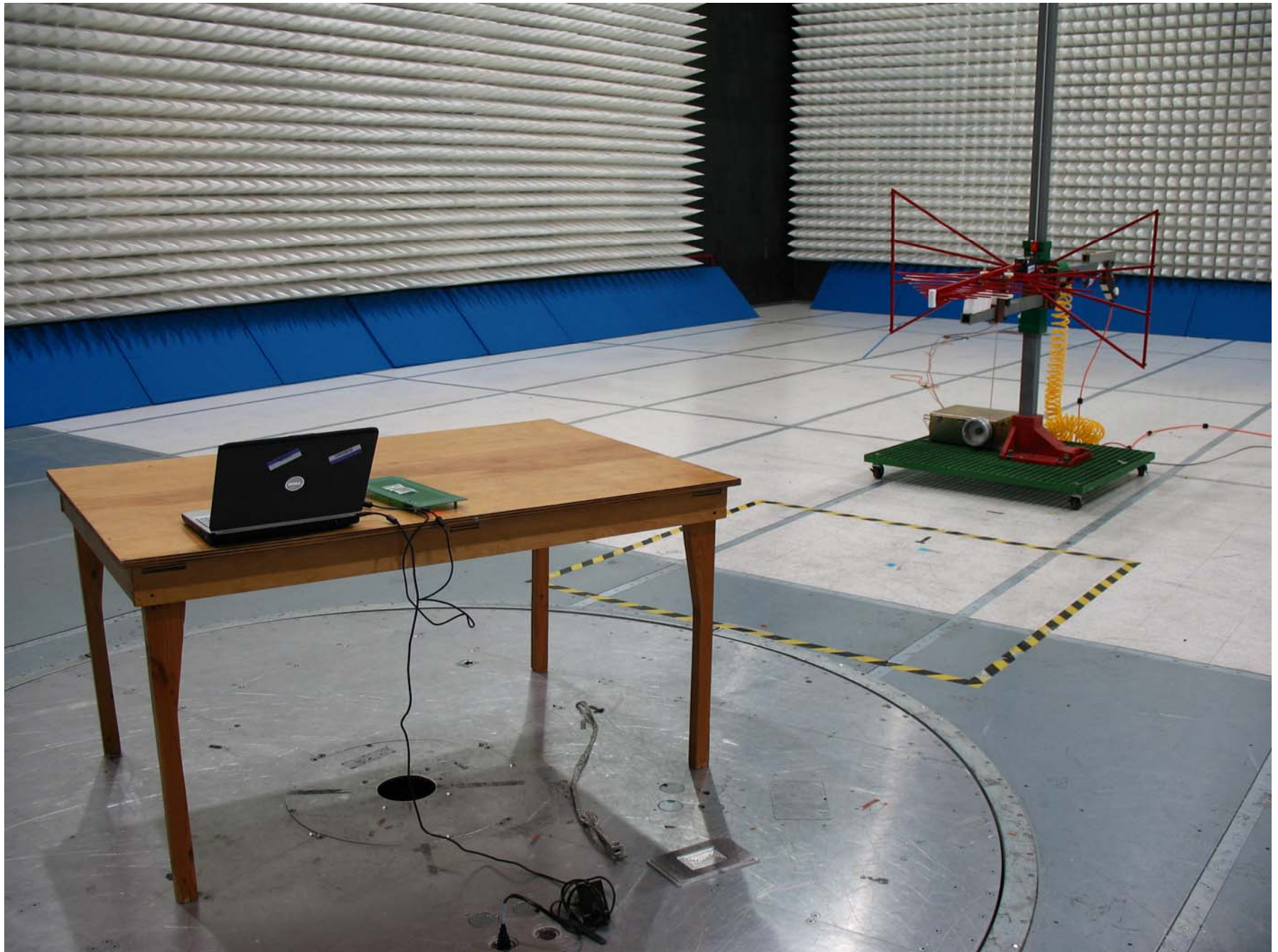
Radiated Emissions (Back)
