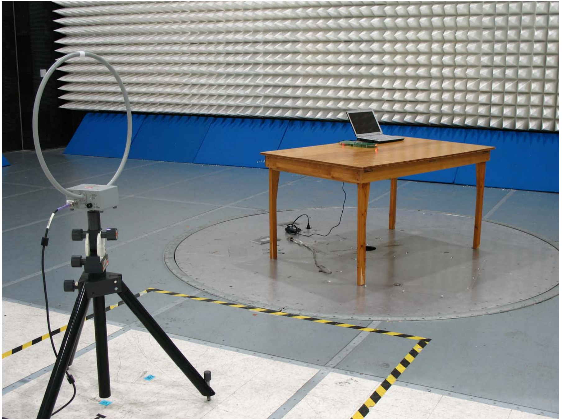
Radiated Emissions (30MHz)
