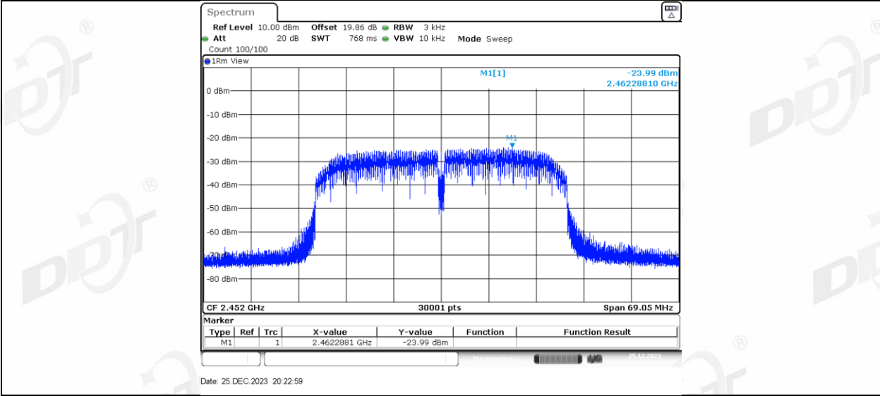
11N40SISO_Ant1_2452
